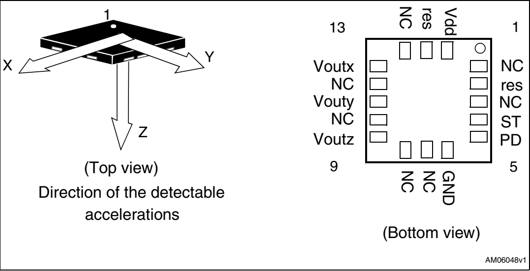
Figure 2. Pin connection
