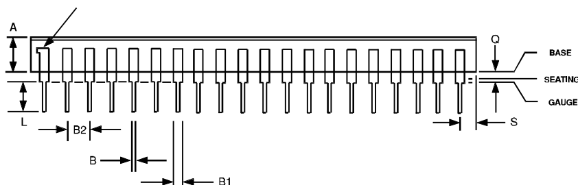
FIGURE 8. MECHANICAL SPECIFICATIONS
