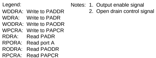
Figure C.6 (b) Port A Block Diagram (Pin PA1)
