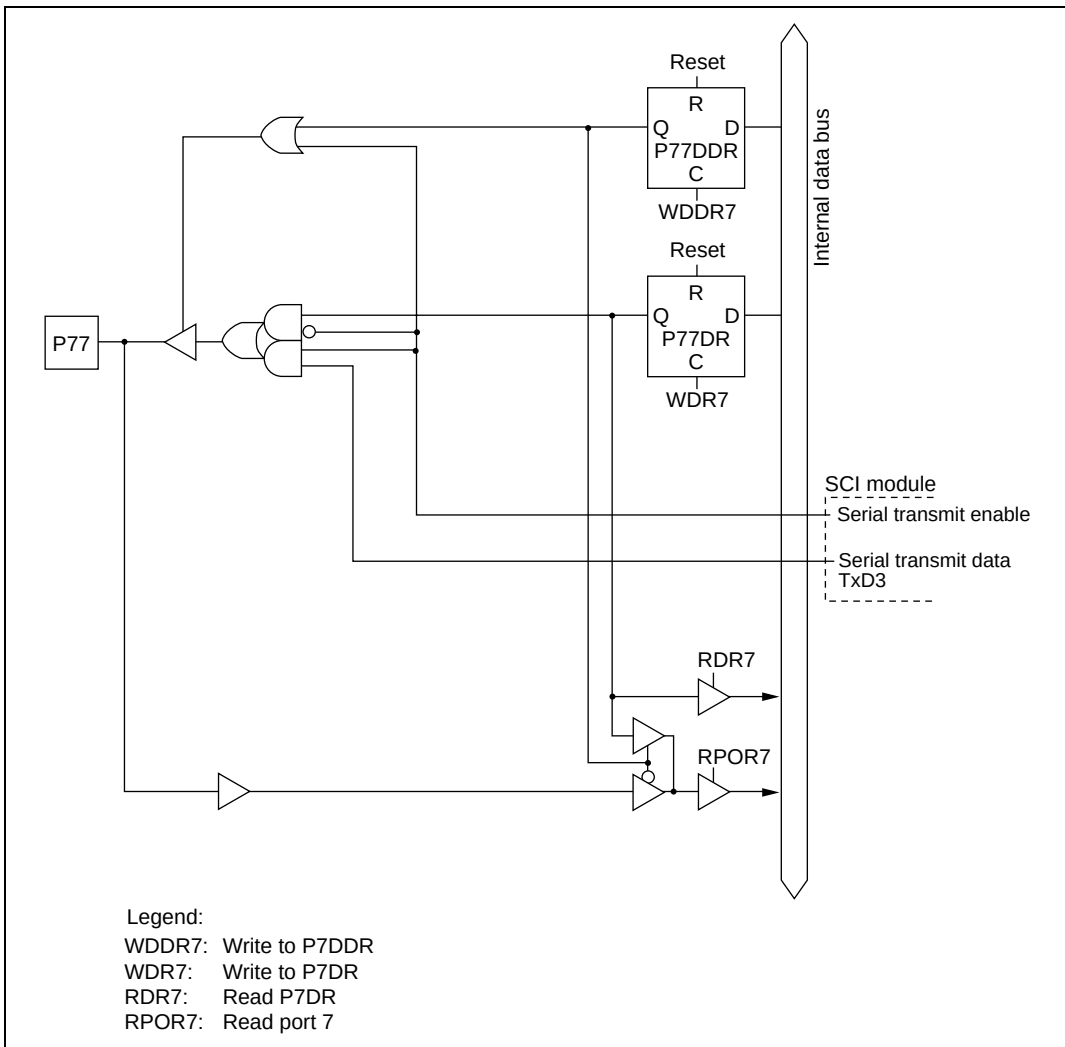
Figure C.16 (e) Port 7 Block Diagram (Pin P77)
