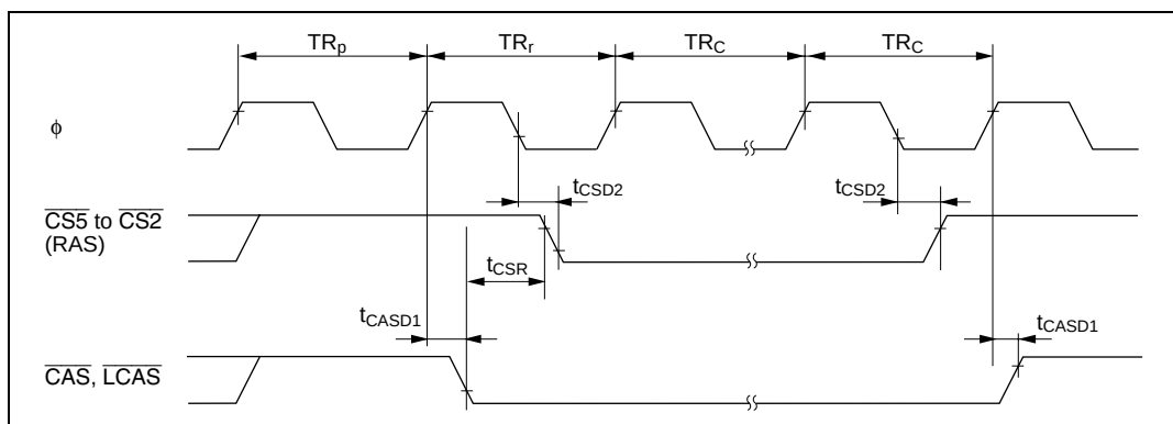
Figure 26.13 DRAM Self-Refresh Timing
