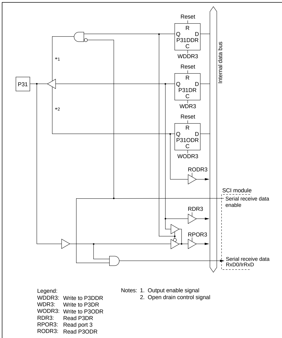
Figure C.14 (b) Port 3 Block Diagram (Pin P31)
