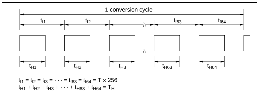
Figure 14.4 (4) Output Waveform
