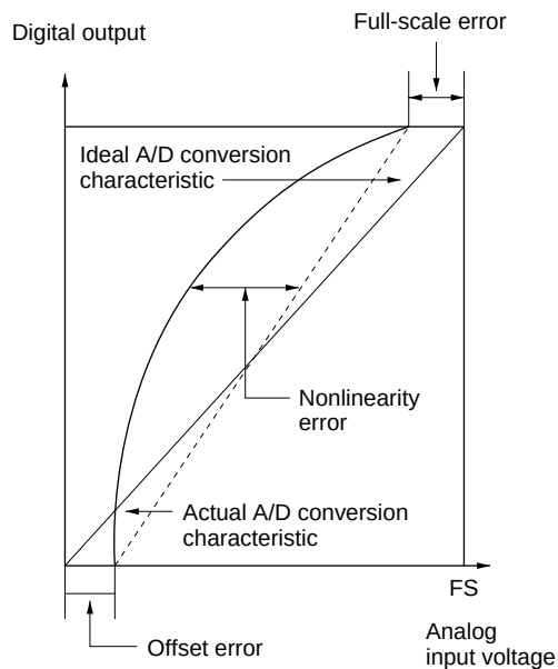
Figure 19.10 A/D Conversion Precision Definitions (2)
