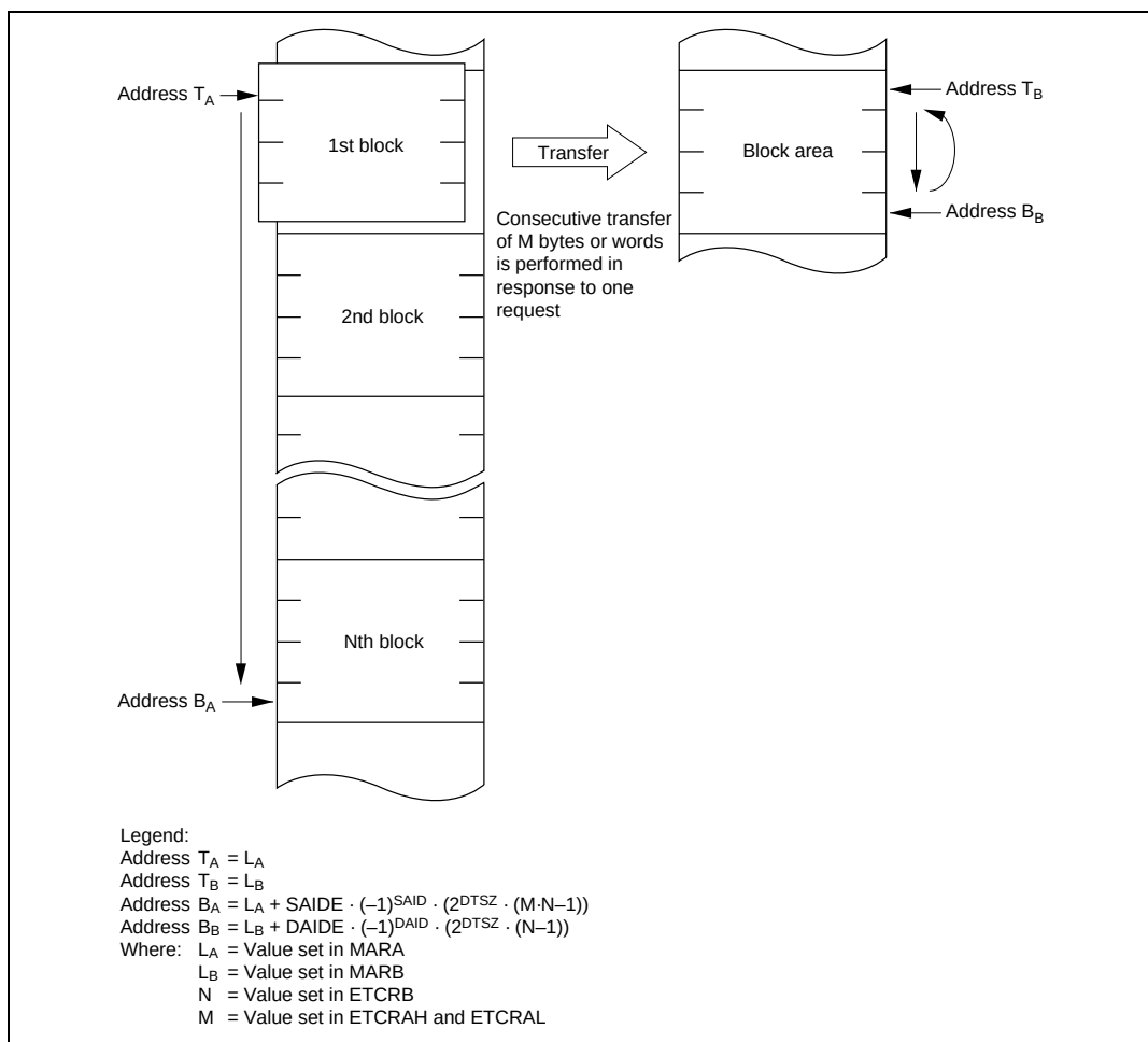
Figure 8.13 Operation in Block Transfer Mode (BLKDIR = 0)
