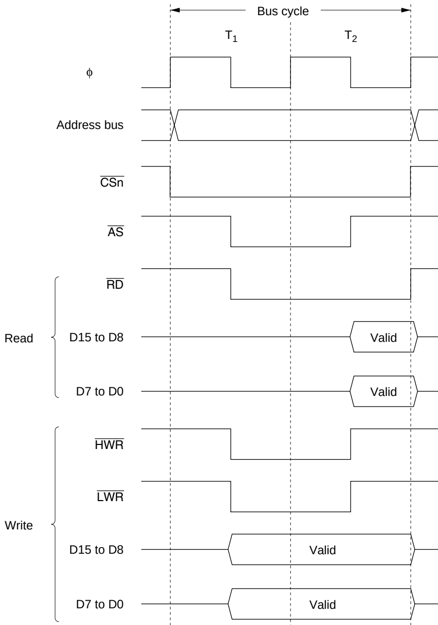
Figure 7.10 Bus Timing for 16-Bit 2-State Access Space (3) (Word Access)
