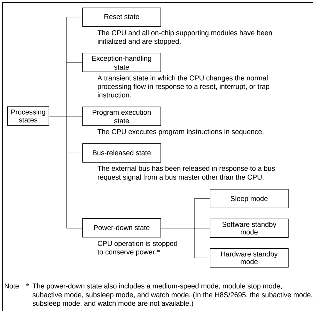
Figure 2.14 Processing States
