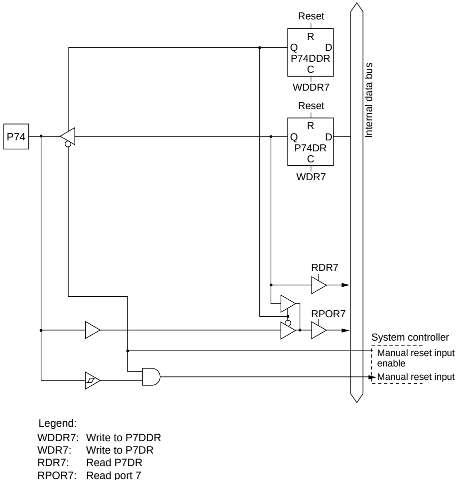
Figure C.16 (b) Port 7 Block Diagram (Pin P74)
