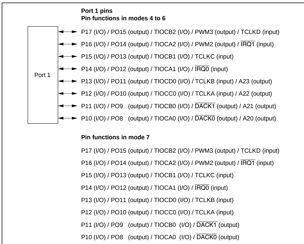
Figure 10A.1 Port 1 Pin Functions
