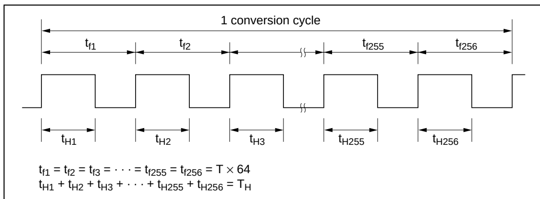
Figure 14.4 (3) Output Waveform
