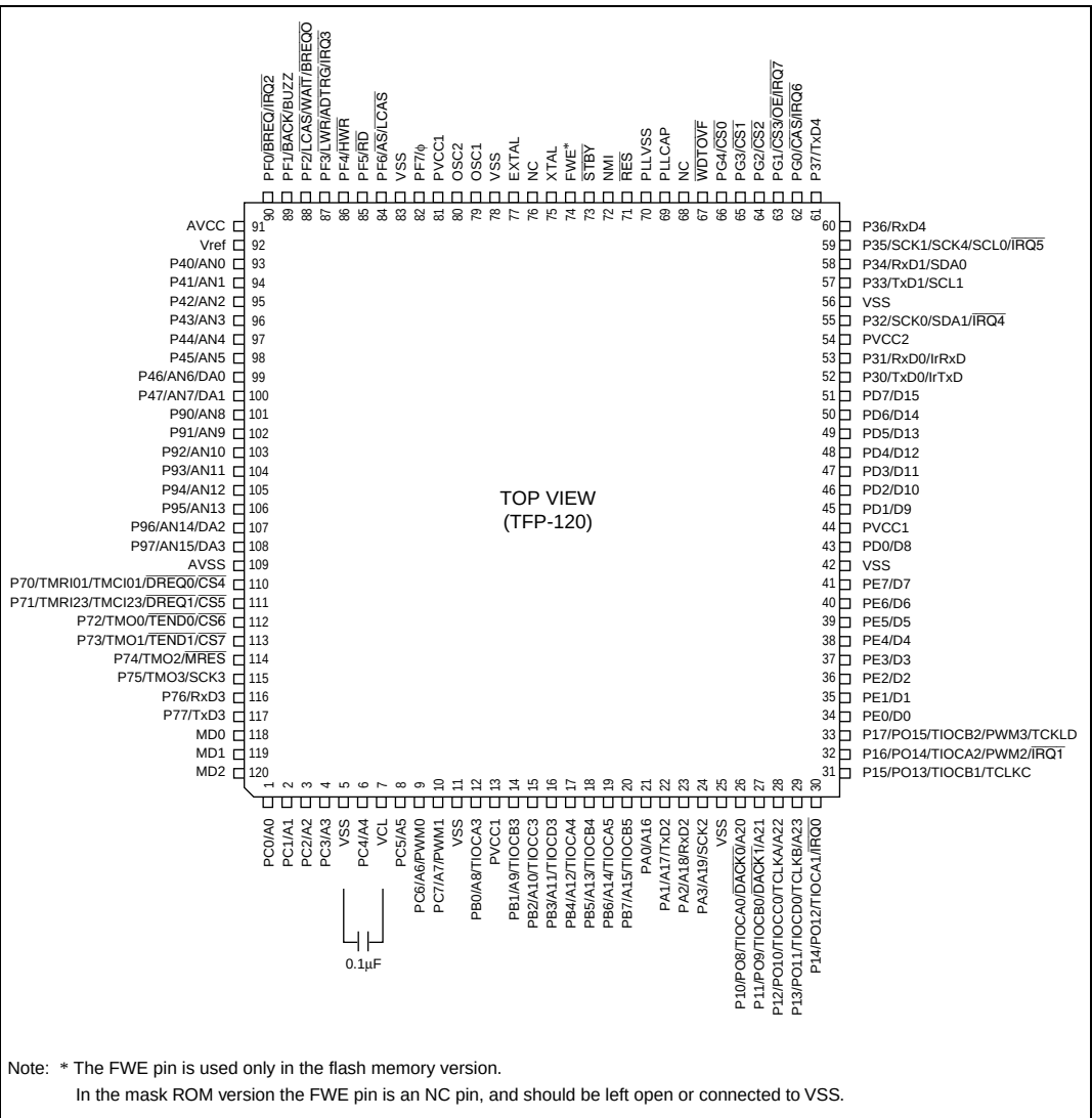
Figure 1.2 (b) H8S/2633R Pin Arrangement (TFP-120: Top View)
