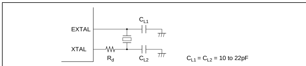
Figure 23A.2 Connection of Crystal Resonator (Example)
