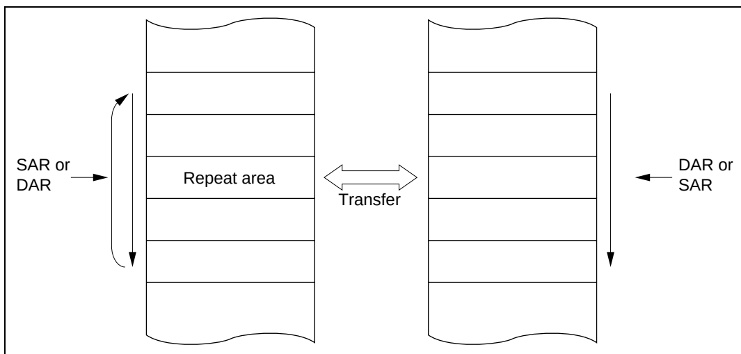
Figure 9.7 Memory Mapping in Repeat Mode
