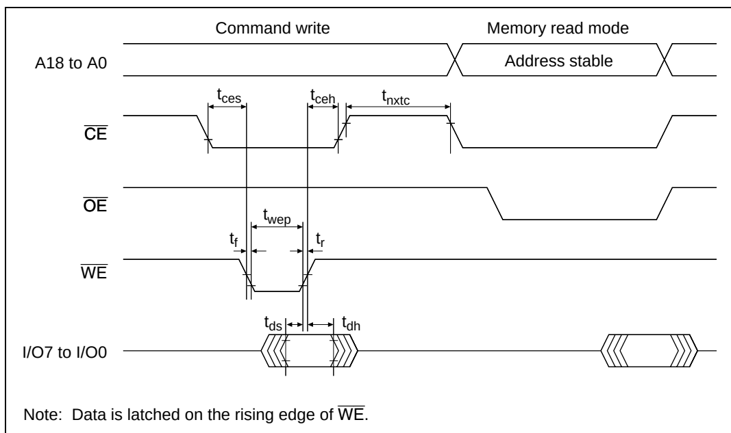
Figure 22.19 Timing Waveforms for Memory Read after Memory Write
