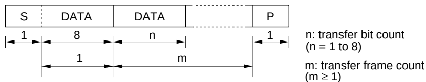
Figure 18.4 I 2 C Bus Data Format (Serial Format)
