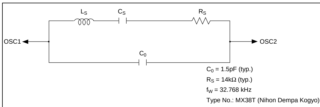
Figure 23A.9 Equivalence Circuit for 32.768kHz Resonator
