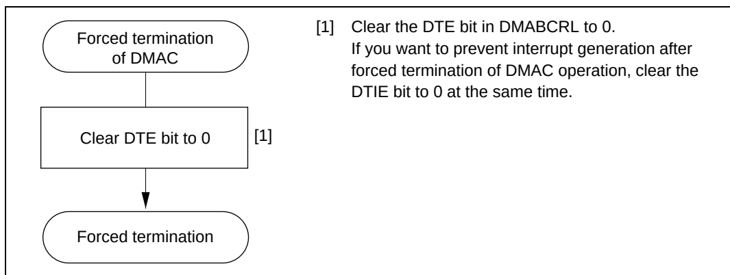
Figure 8.37 Example of Procedure for Forcibly Terminating DMAC Operation
