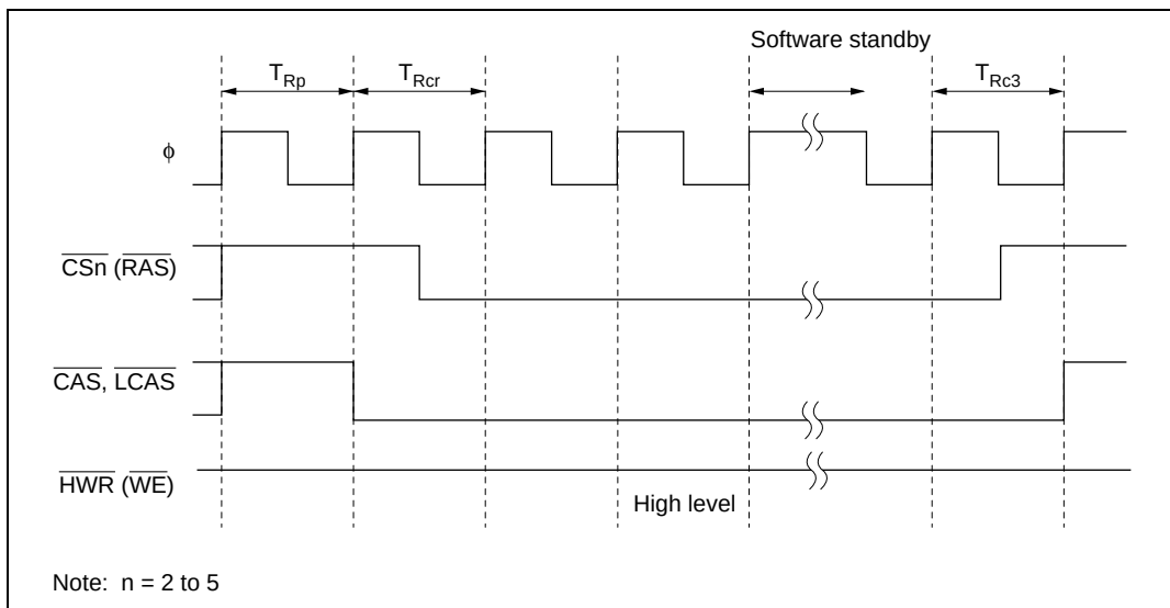
Figure 7.29 Self-Refresh Timing
