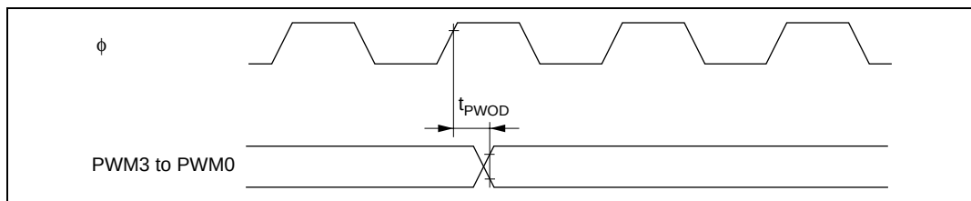
Figure 26.29 PWM Output Timing
