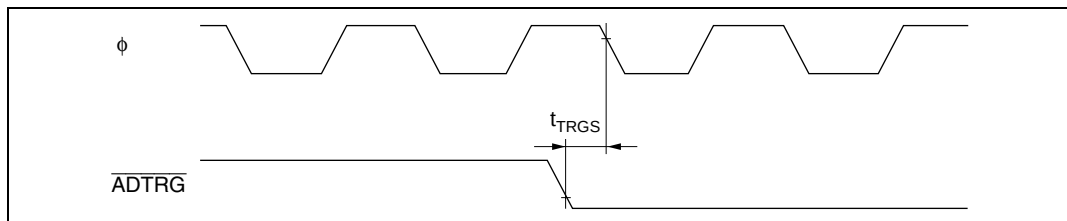
Figure 27.19 A/D Converter External Trigger Input Timing
