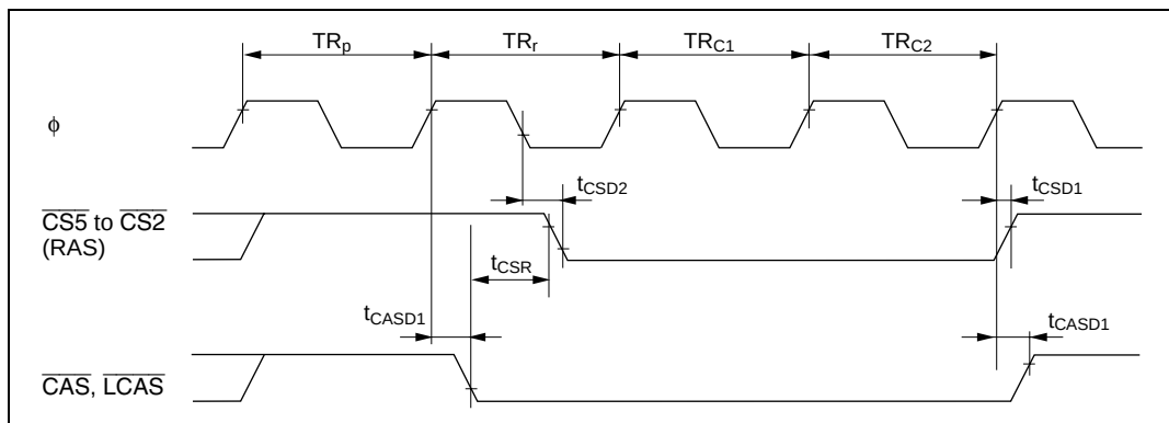
Figure 26.12 DRAM CBR Refresh Timing
