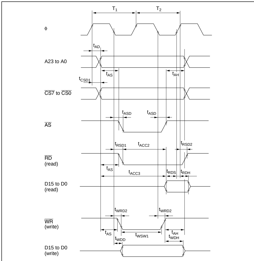
Figure 25.6 Basic Bus Timing (Two-State Access)
