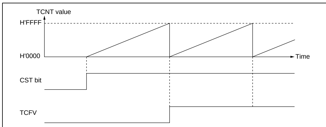
Figure 11.7 Free-Running Counter Operation
