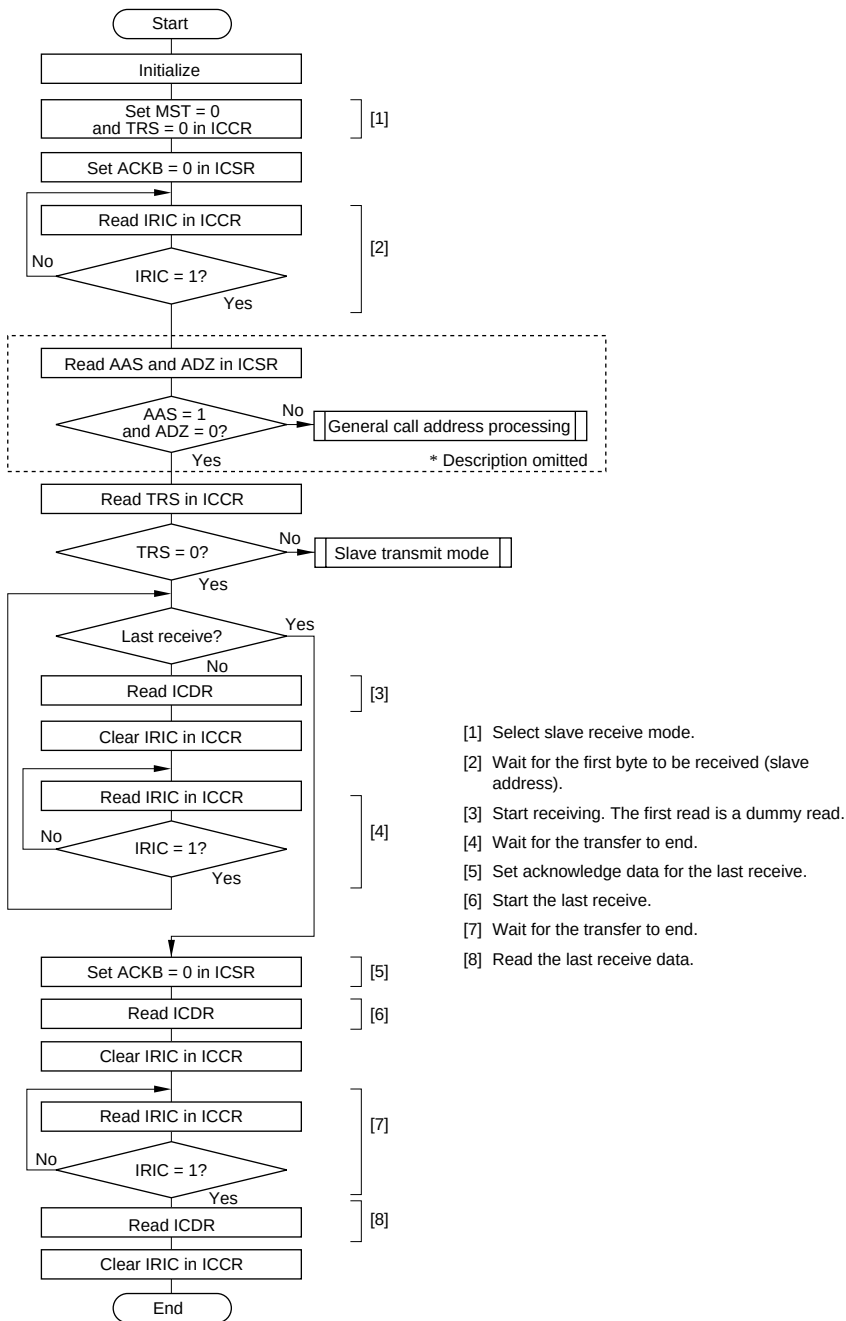
Figure 18.19 Flowchart for Slave Transmit Mode (Example)
