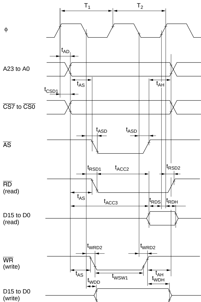
Figure 27.6 Basic Bus Timing (Two-State Access)
