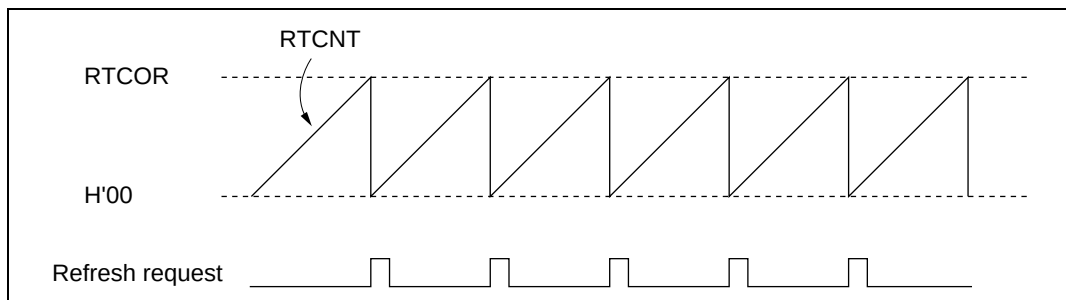
Figure 7.25 RTCNT Operation
