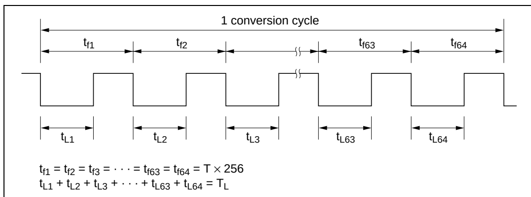
Figure 14.4 (2) Output Waveform
