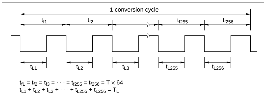
Figure 14.4 (1) Output Waveform
