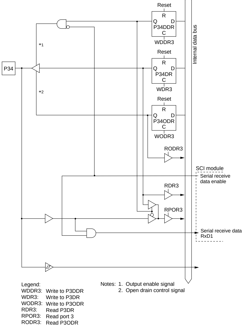
Figure C.14 (e) Port 3 Block Diagram (Pin P34)
