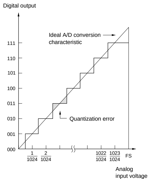
Figure 19.9 A/D Conversion Precision Definitions (1)
