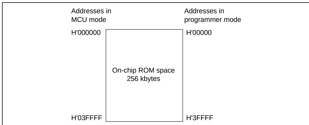
Figure 22.18 On-Chip ROM Memory Map
