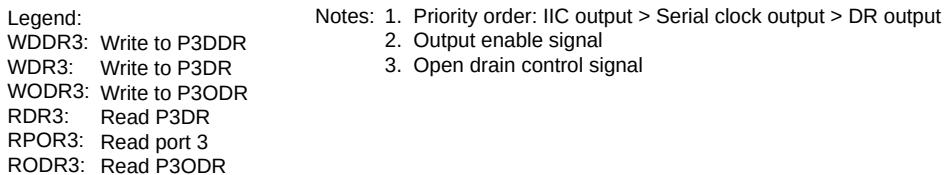
Figure C.2 (c) Port 3 Block Diagram (Pin P32)
