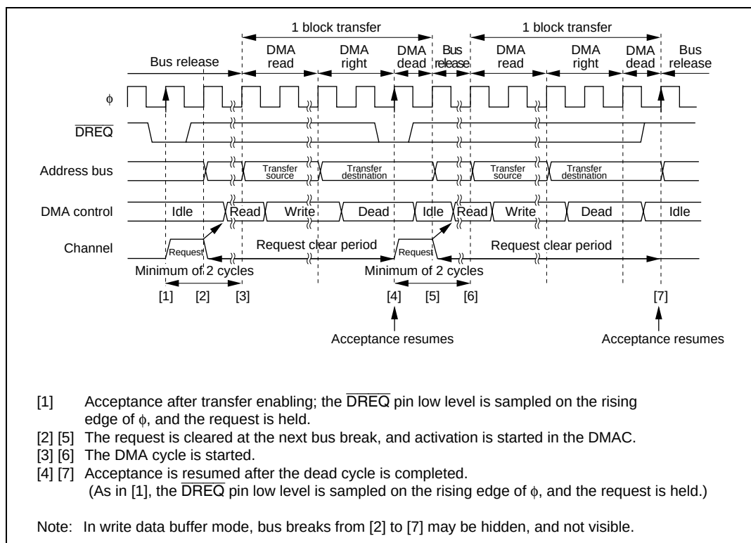
Figure 8.26 Example of \overline{\text{DREQ}} Level Activated Block Transfer Mode Transfer
