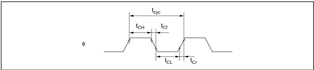
Figure 25.2 System Clock Timing
