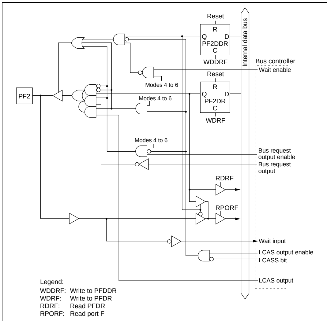
Figure C.11 (c) Port F Block Diagram (Pin PF2)
