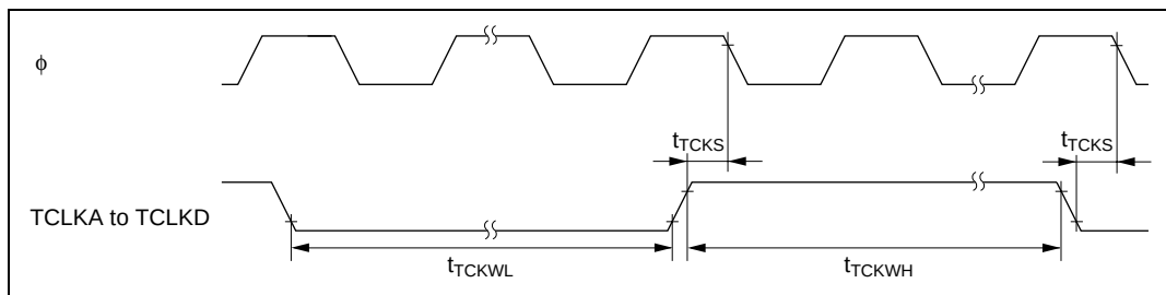
Figure 26.23 TPU Clock Input Timing
