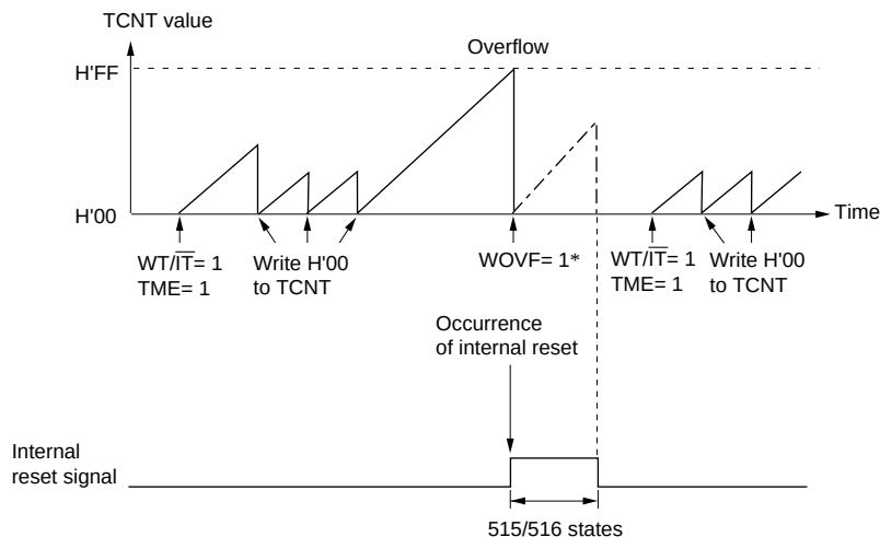
Figure 15.4 (a) WDT0 Watchdog Timer Operation
