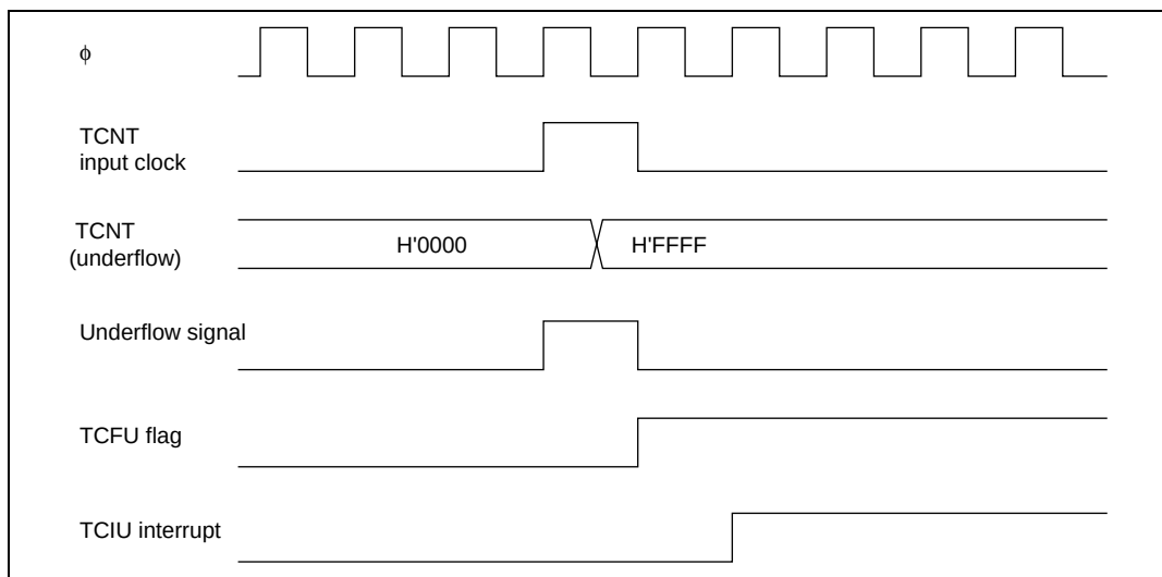
Figure 11.45 TCIU Interrupt Setting Timing
