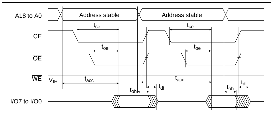
Figure 22.22 \overline{\text{CE}} and \overline{\text{OE}} Clock System Read Timing Waveforms
