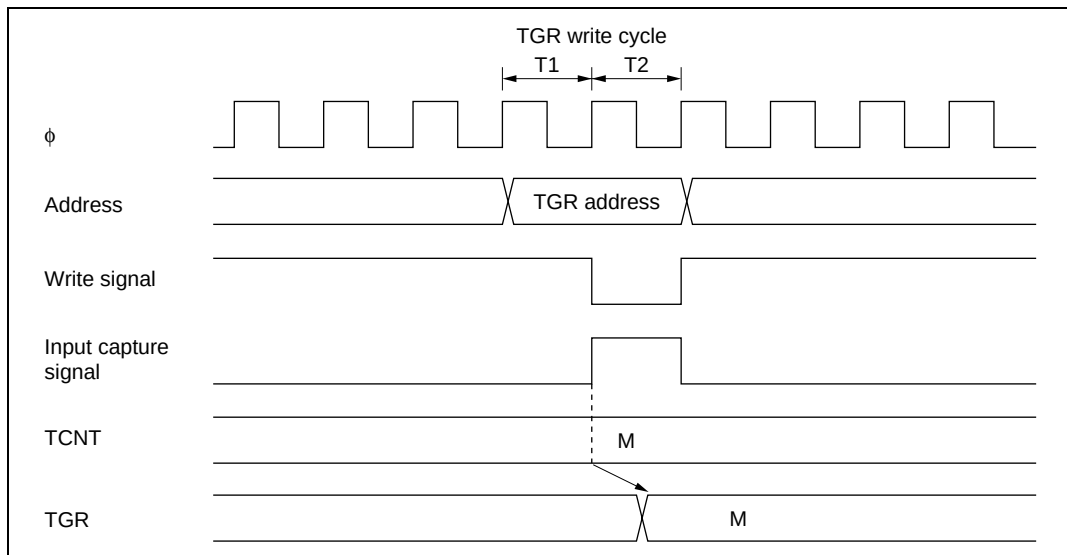
Figure 11.54 Contention between TGR Write and Input Capture
