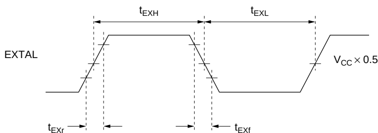
Figure 23A.7 External Clock Input Timing
