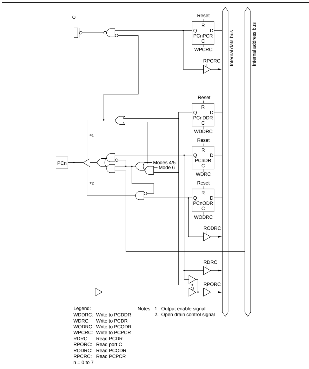
Figure C.20 Port C Block Diagram (Pins PC0 to PC7)
