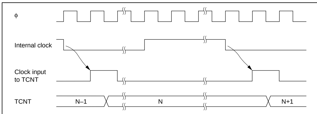
Figure 13.2 Count Timing for Internal Clock Input
