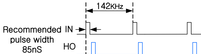
Figure 4c. Recommendation of pulse width Output Waveform
