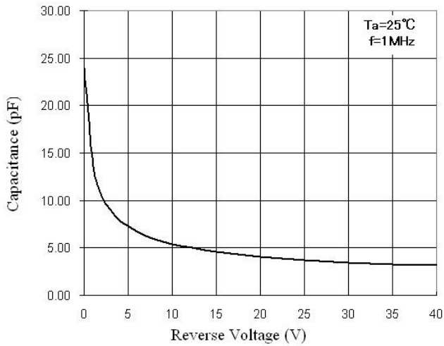
Fig.1 Total Capacitance
