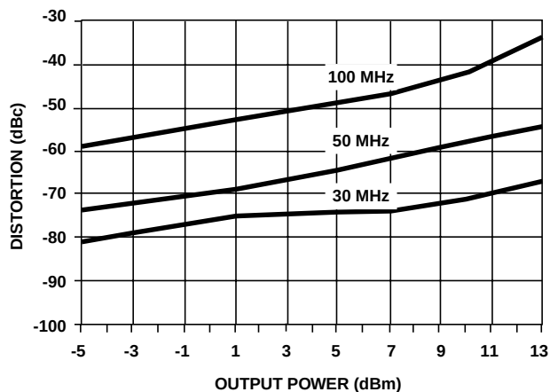
FIGURE 13. 2ND HARMONIC DISTORTION vs P_{\text{OUT}}
