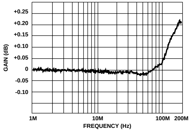
FIGURE 9. GAIN FLATNESS
