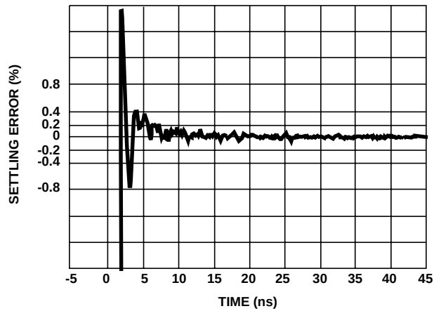
FIGURE 15. SETTLING RESPONSE ( V_{\text{OUT}} = 1\text{V} )
