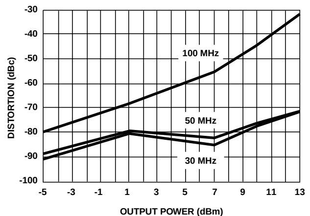
FIGURE 14. 3RD HARMONIC DISTORTION vs P_{\text{OUT}}
