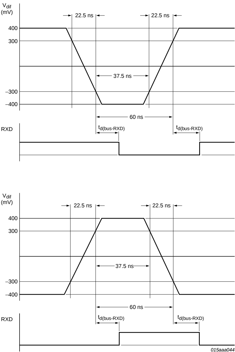
Fig 13. Receiver test signal
