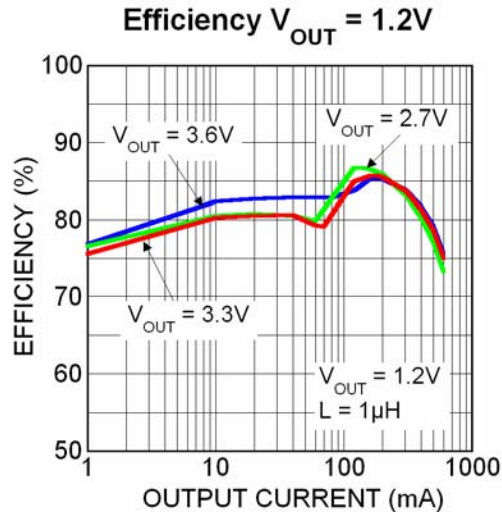
Figure 1. MIC23050 Efficiency Curve
