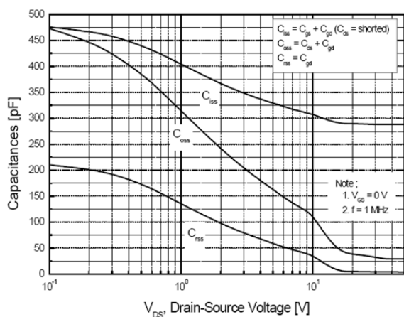
Fig. 5 Capacitance Characteristics
