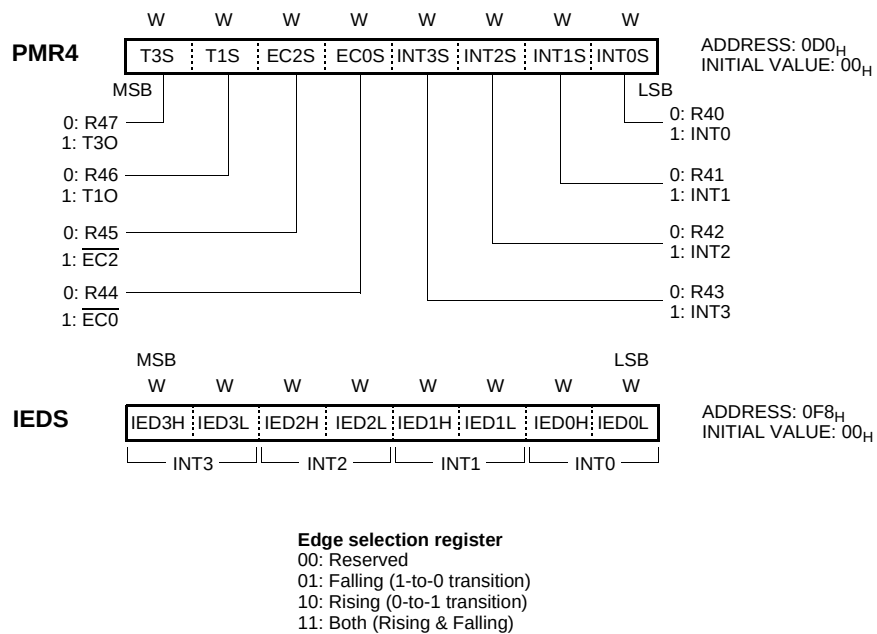
Figure 16-9 PMR4 and IEDS Registers
