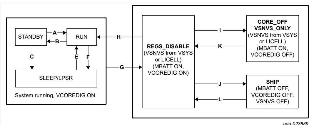
Figure 26. PMIC state machine
