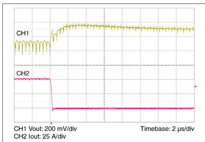
Figure 11 — 50-0 A load step with 100 \mu F input capacitor and no output capacitor.
