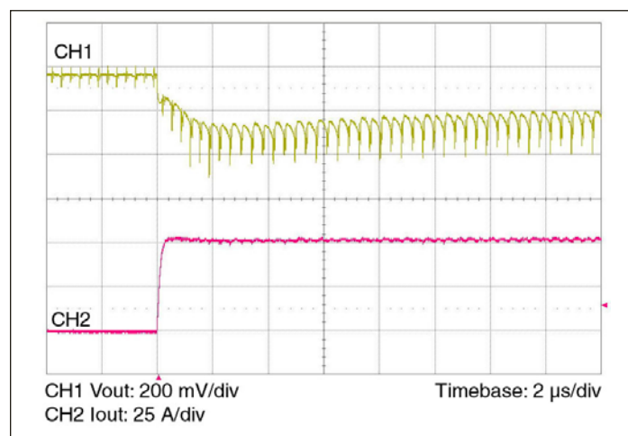
Figure 10 — 0-50 A load step with 100 \mu F input capacitor and no output capacitor.
