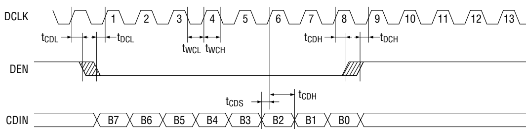
Figure 2 MCU Interface Timing Diagram
