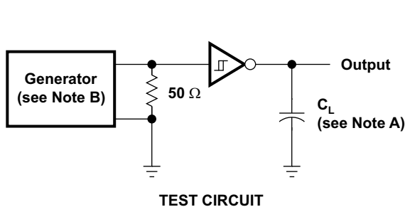
Figure 7. Driver Pulse Skew
