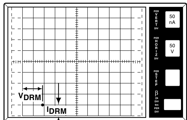
Figure AN1006.22 I_{DRM} = 50 \text{ nA} at V_{DRM} = 90 \text{ V}
