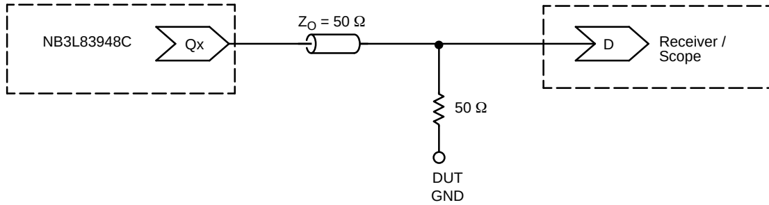
Figure 5. Typical Termination for Output Driver and Device Evaluation. Supplies may be centered on GND ( \pm 1.65\text{ V} or \pm 1.25\text{ V} ) to permit direct connection into 50\ \Omega to GND Scope modules
