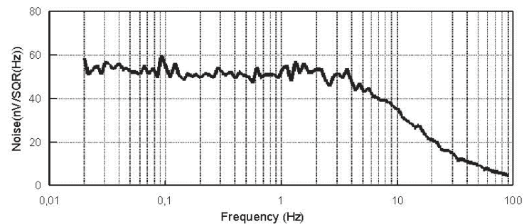
Noise = F(frequency)
