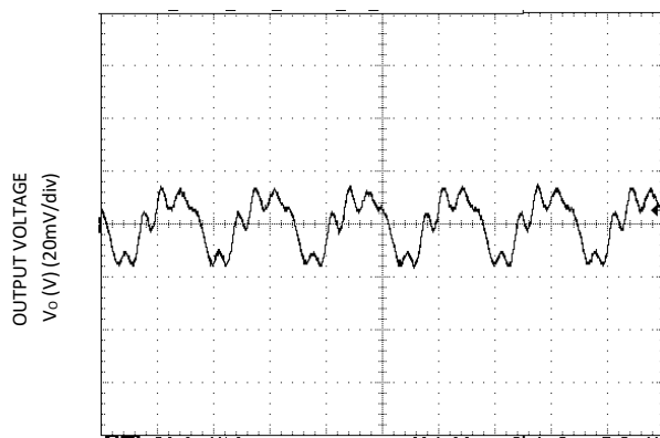
TIME, t (1 \mu s/div) V_o=3.3V , I_o = I_{o,max}
