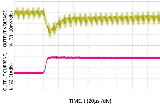
Transient Response to Dynamic Load Change from 50% to 100% at 12Vin, Cout= 1x47uF +1x330uF, CTune=10nF & RTune=267. Vo=1.8V
