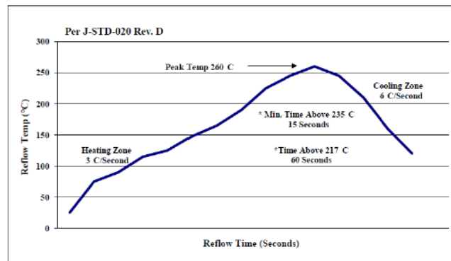
Figure 51. Recommended linear reflow profile using Sn/Ag/Cu solder.
