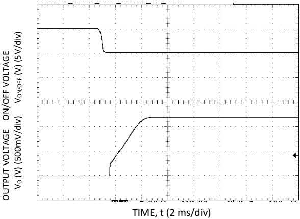
Start-up Using On/Off Voltage ( I_o = I_{o,max} ), V_o=1.2V
