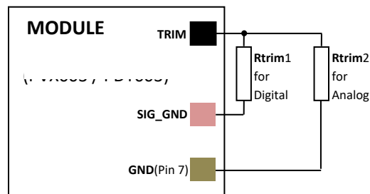
Figure 46. Layout to support either Analog or Digital on the same pad.
