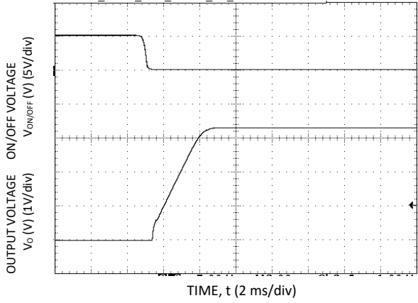
Start-up Using On/Off Voltage ( I_o = I_{o,max} ), V_o=3.3V
