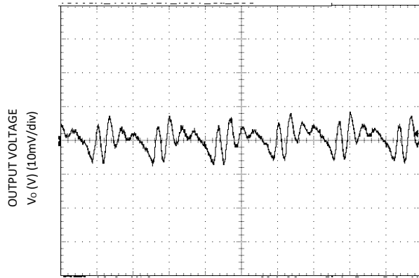
TIME, t (1 \mu s/div) V_o=0.6V , I_o = I_{o,max}
