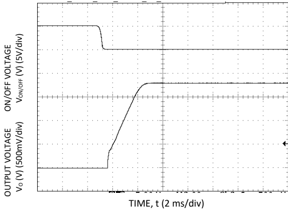
Start-up Using On/Off Voltage ( I_o = I_{o,max} ), V_o=1.8V
