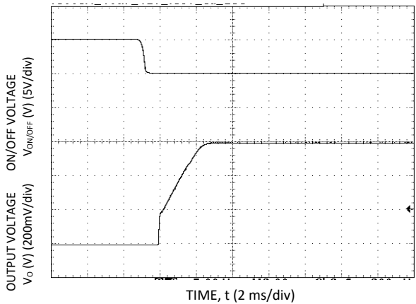
Start-up Using On/Off Voltage ( I_o = I_{o,max} ), V_o=0.6V
