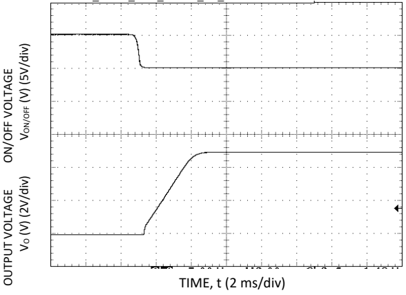
Start-up Using On/Off Voltage ( I_o = I_{o,max} ), V_o=5.0V
