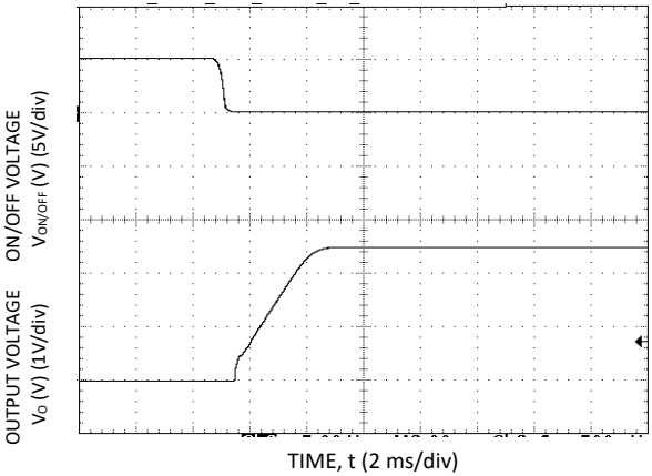
Start-up Using On/Off Voltage ( I_o = I_{o,max} ), V_o=2.5V
