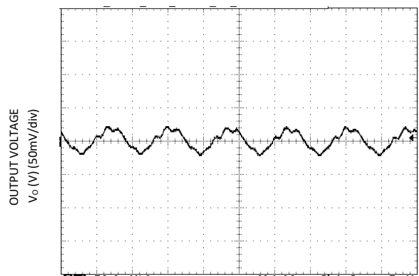
TIME, t (1 \mu s/div) V_o=5.0V , I_o = I_{o,max}
