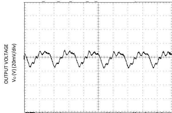
TIME, t (1 \mu s/div) V_o=2.5V , I_o = I_{o,max}
