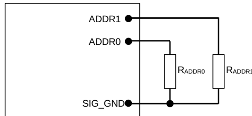
Figure 48. Circuit showing connection of resistors used to set the Power Management Bus address of the module.
