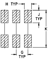
Suggested Layout, Tolerance to be within ±0.02
