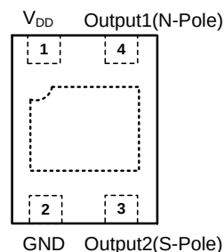
X2-DFN1410-4
