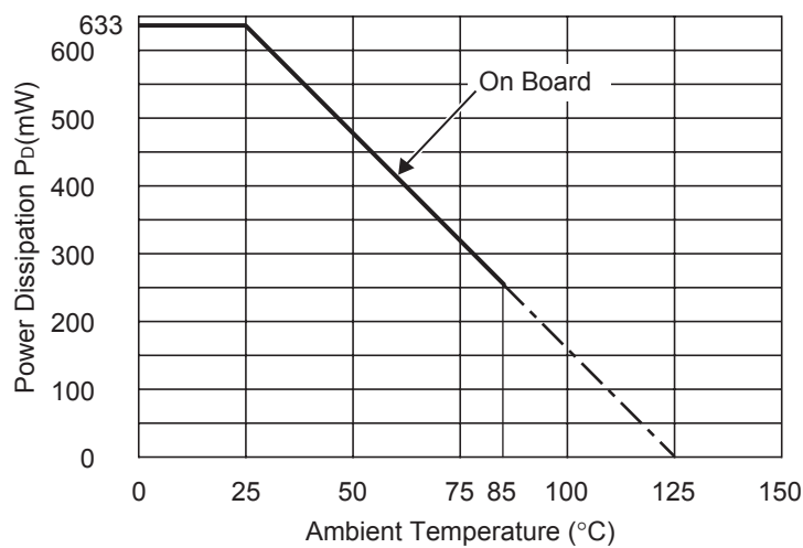
Power Dissipation
