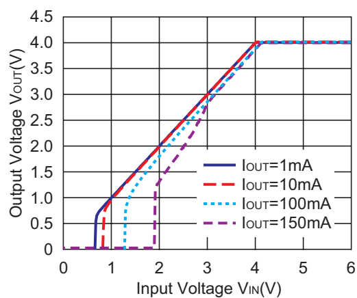
4.0V(VR1/VR2)
