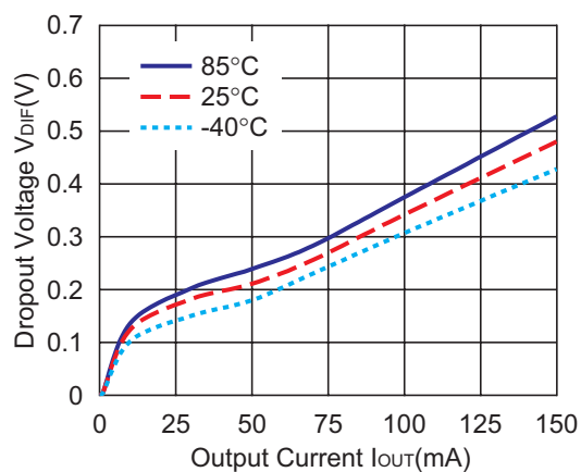
1.0V(VR1/VR2)
