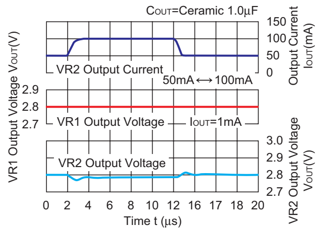
2.8V(VR1/VR2)
