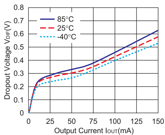
0.9V(VR1/VR2)
