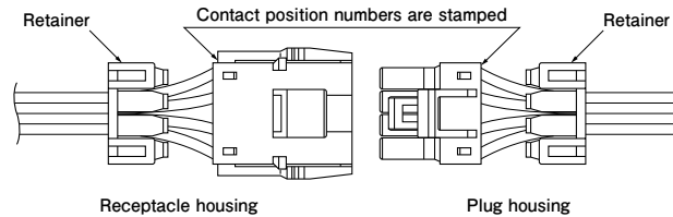
Receptacle housing
