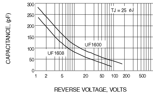
Fig. 4-TYPICAL JUNCTION CAPACITANCE
