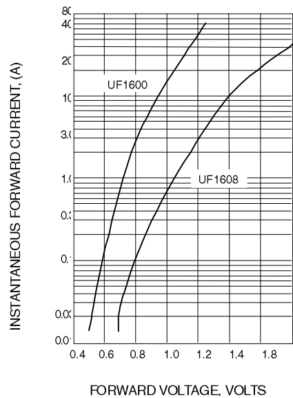
Fig. 5-TYPICAL FORWARD CHARACTERISTICS
