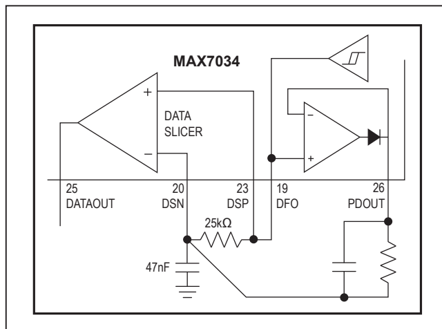
Figure 4. Using PDOUT for Faster Startup
