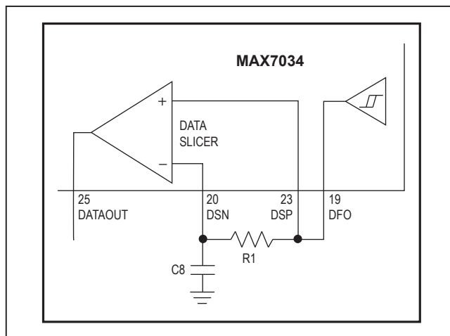
Figure 2. Generating Data Slicer Threshold
