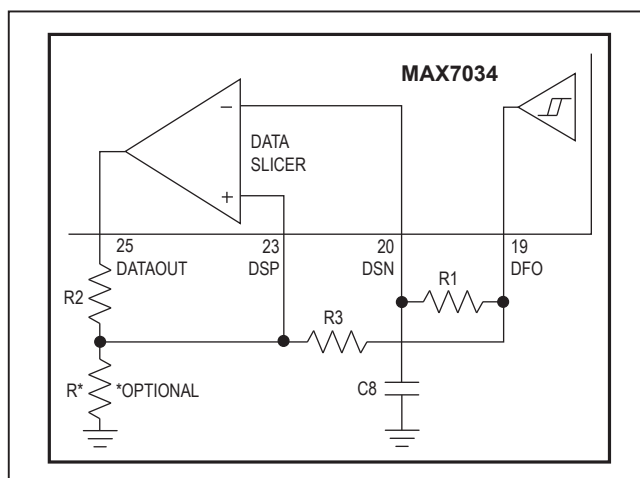
Figure 3. Generating Data Slicer Hysteresis
