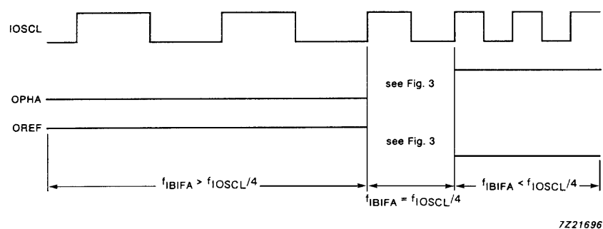
Fig.4 Generation of phase output signal (OPHA) and phase reference signal (OREF); f_{IBIFA} = f_{IOSCL}/4 .
