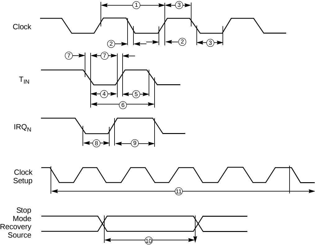
Figure 5. Timing Diagram
