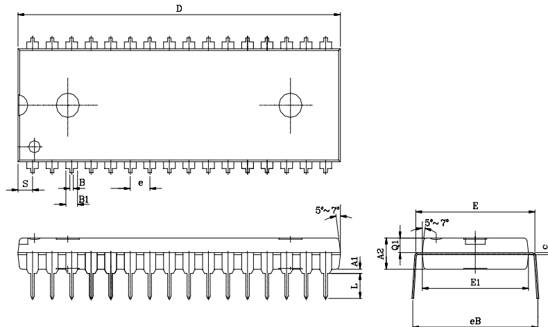
PDIP - 32
