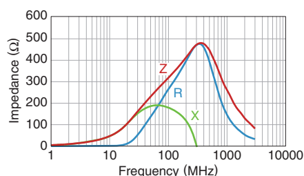
KMZ1608YHR301BTD25
