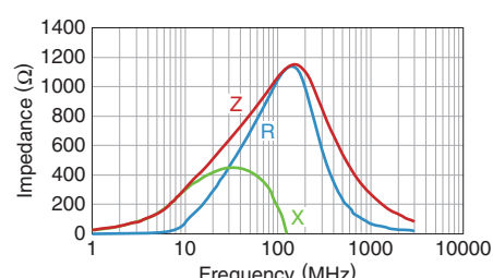
KMZ1608SHR102ATD25
