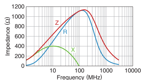
KMZ1608BHR102CTD25
