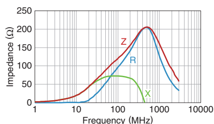
KMZ1608YHR121BTD25
