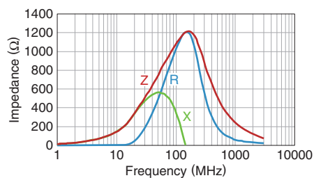
KMZ1608YHR102BTD25
