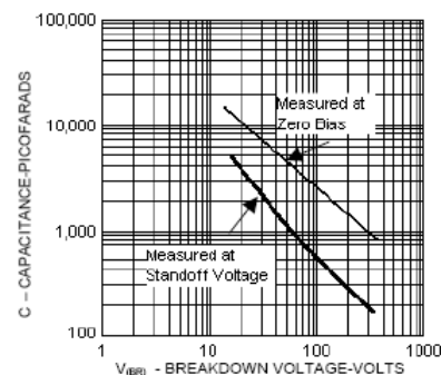
FIGURE 3 Typical Capacitance vs. Breakdown Voltage
