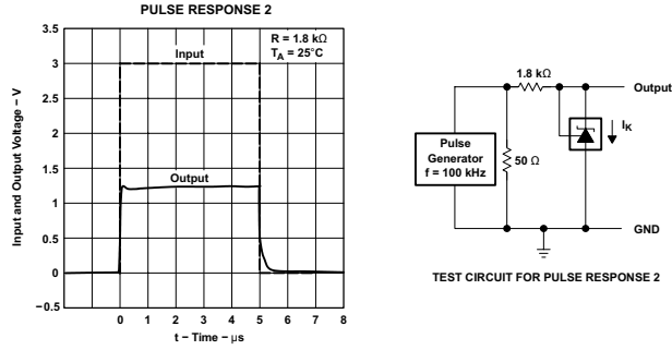
图 6-13. Pulse Response 2
