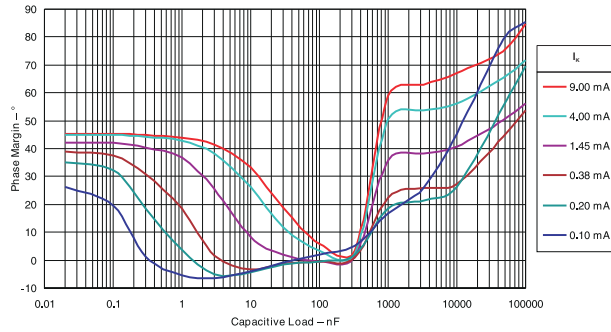
图 6-15. Phase Margin vs Capacitive Load V_{KA} = V_{REF} (1.25 V), T_A = 25^\circ\text{C}
