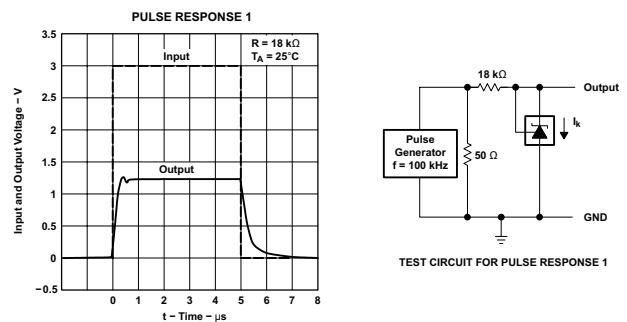
图 6-12. Pulse Response 1
