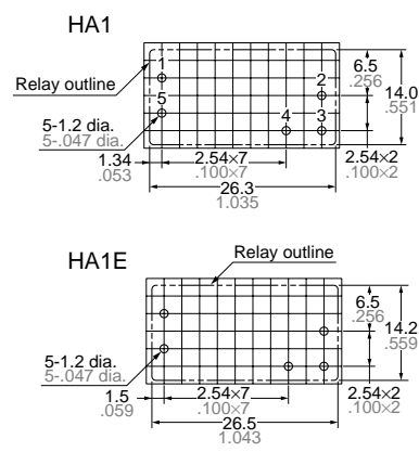
PC board pattern (Copper-side view)
