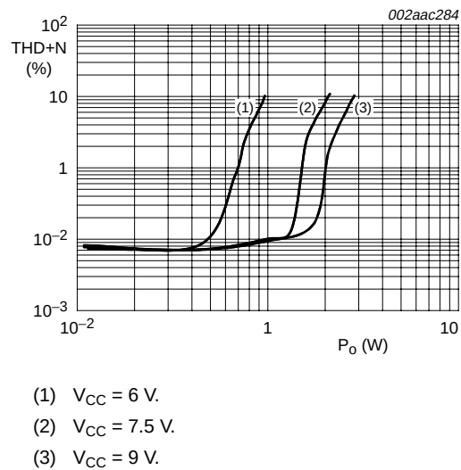
Fig 15. Total harmonic distortion-plus-noise as a function of output power
