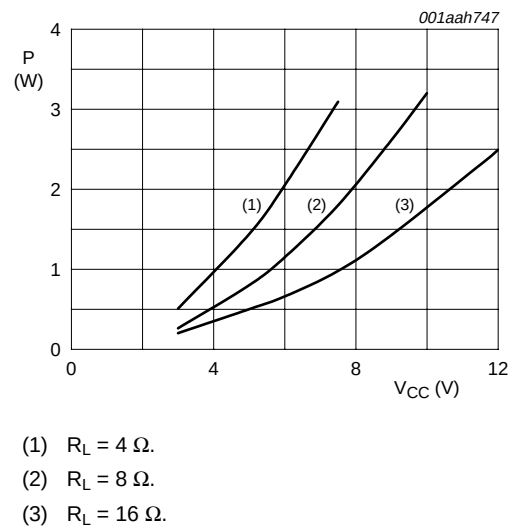
Fig 13. Worst case power dissipation as a function of supply voltage
