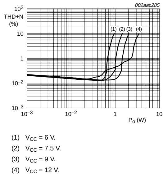
Fig 15. Total harmonic distortion-plus-noise as a function of output power
