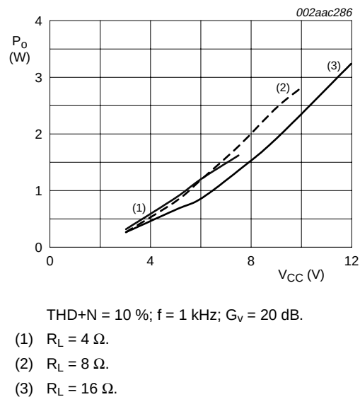
Fig 14. Output power as a function of supply voltage
