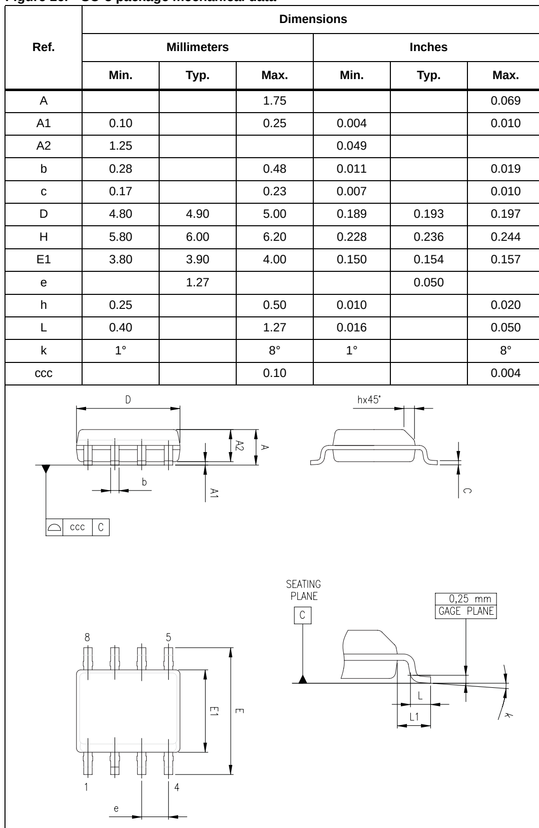
Figure 16. SO-8 package mechanical data
