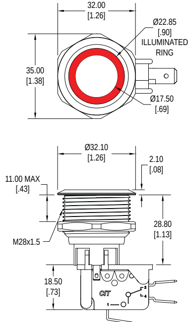
B - Flush, Ring Illuminated
