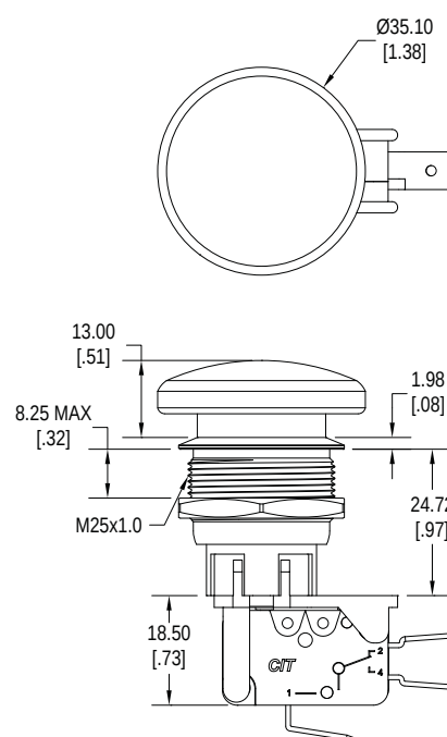
MR - Mushroom Actuator
