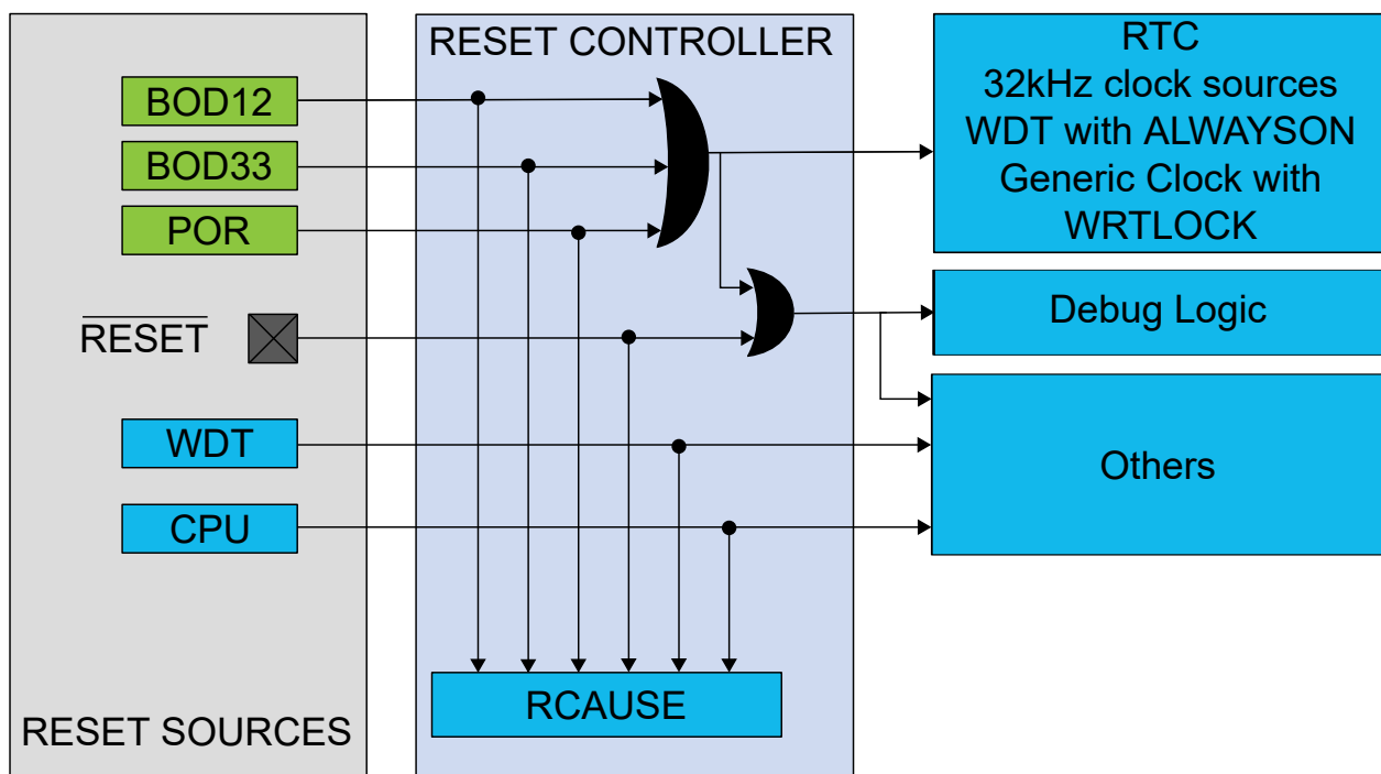
Figure 16-3. Reset Controller
