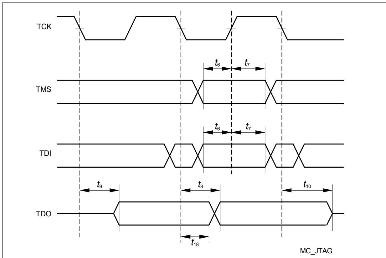
Figure 23 JTAG Timing
