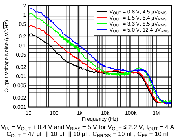
图 12. Output Noise vs Frequency and V_{OUT}
