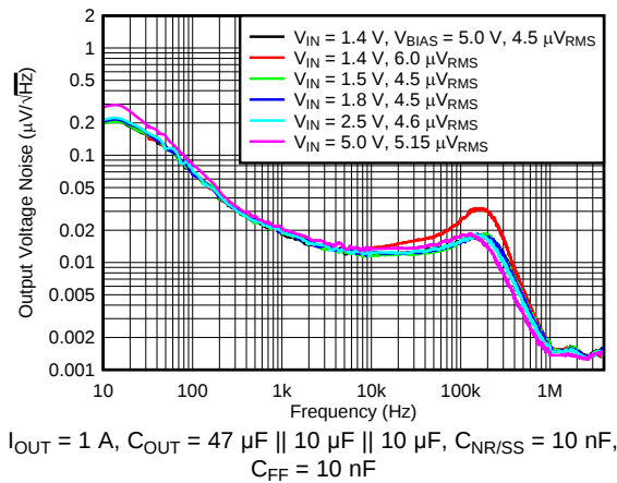
图 13. Output Noise vs Frequency and V_{IN}
