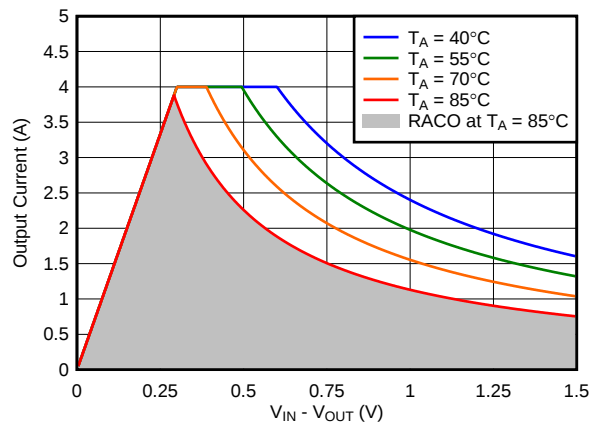
图 63. Recommended Area for Continuous Operation for V_{OUT} = 3.3\text{ V}
