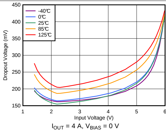
图 23. Dropout Voltage vs Input Voltage without Bias
