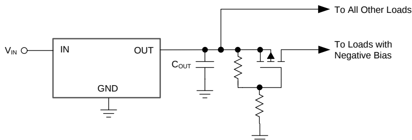
图 56. PMOSFET to Isolate the Output from the Load
