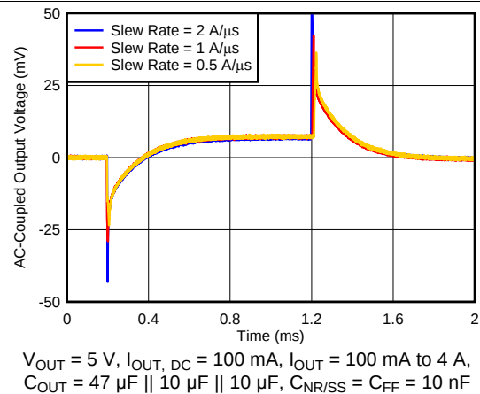
图 20. Load Transient Waveform vs Time and Slew Rate
