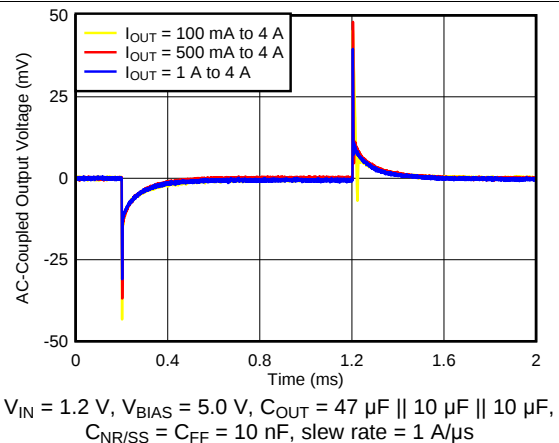
图 22. Load Transient Waveform vs Time and DC Load ( V_{OUT} = 0.9\text{ V} )
