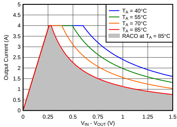
图 61. Recommended Area for Continuous Operation for V_{OUT} = 1.8\text{ V}
