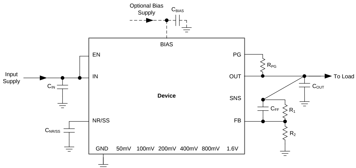
图 49. Adjustable Operation
