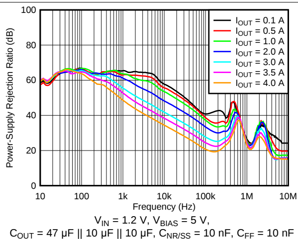
图 1. PSRR vs Frequency and I_{OUT}
