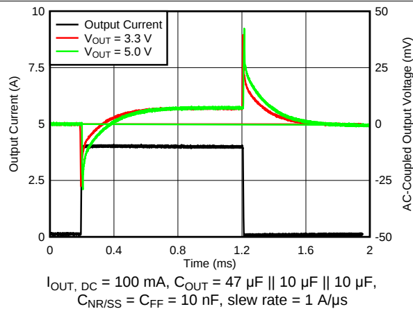
图 19. Load Transient Waveform vs Time and V_{OUT} without Bias
