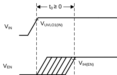
图 50. Sequencing Diagram
