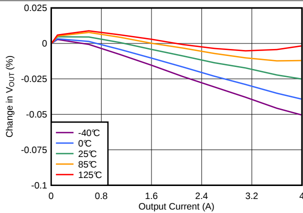
图 31. Load Regulation (5-V Output)
