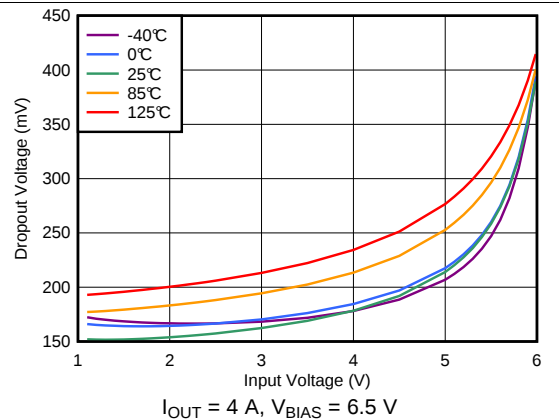
图 24. Dropout Voltage vs Input Voltage with Bias
