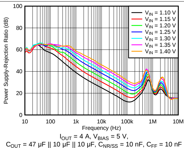
图 2. PSRR vs Frequency and V_{IN} with Bias
