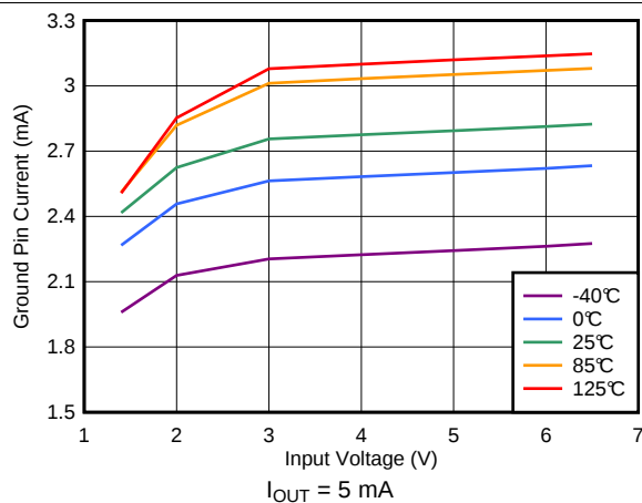
图 35. Ground Pin Current vs Input Voltage
