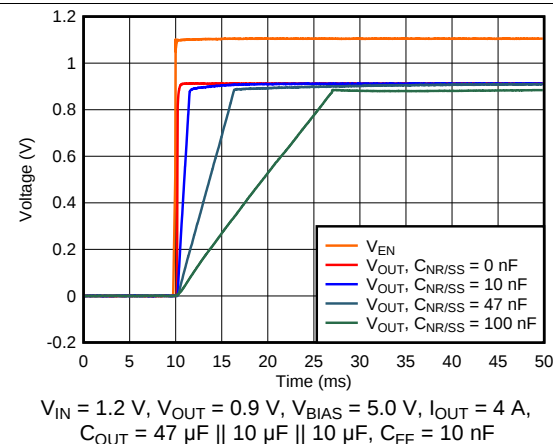
图 17. Start-Up Waveform vs Time and C_{NR/SS}
