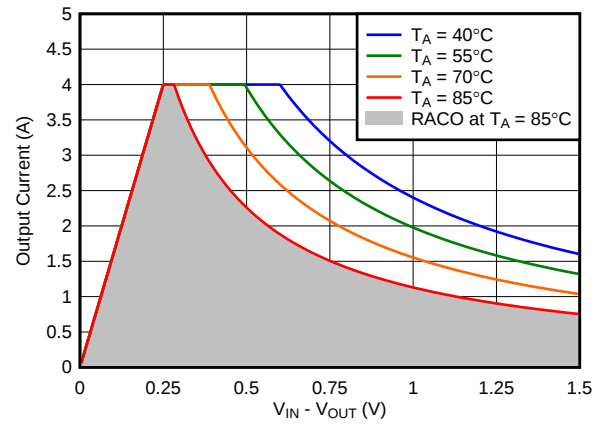
图 60. Recommended Area for Continuous Operation for V_{OUT} = 1.2\text{ V} with Bias
