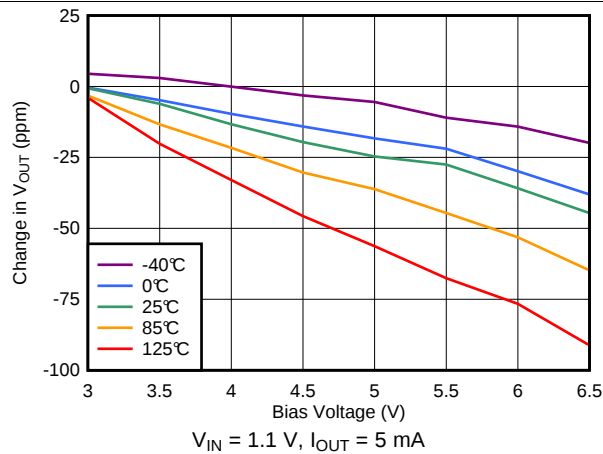
图 33. Line Regulation vs Bias Voltage
