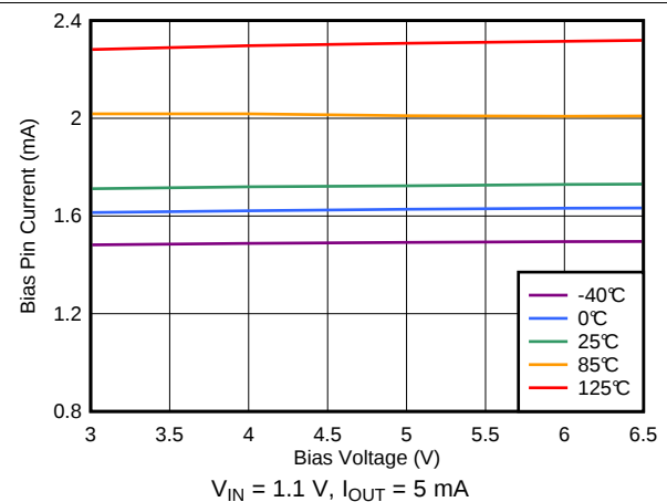
图 36. Bias Pin Current vs Bias Voltage
