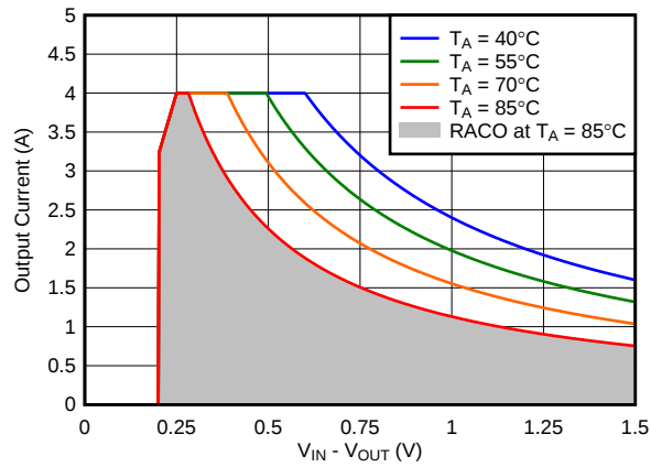
图 59. Recommended Area for Continuous Operation for V_{OUT} = 0.9\text{ V} with Bias
