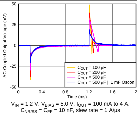
图 21. Load Transient Waveform vs Time and C_{OUT} ( V_{OUT} = 0.9\text{ V} )
