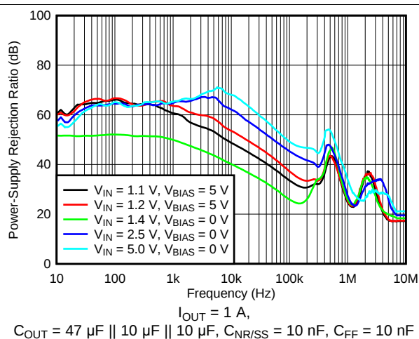
图 4. PSRR vs Frequency and V_{IN}
