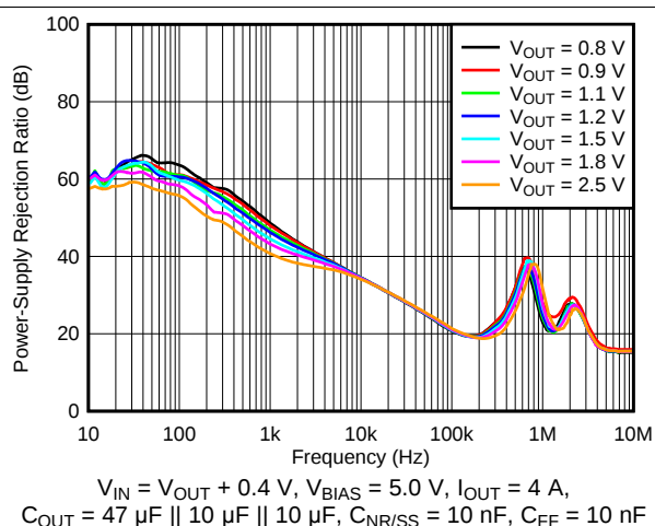
图 5. PSRR vs Frequency and V_{OUT} with Bias
