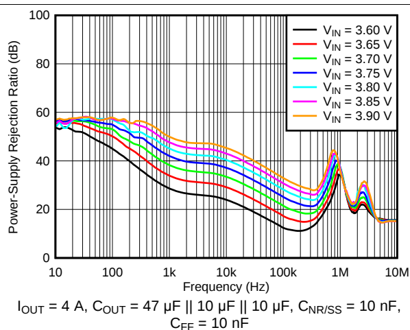
图 6. PSRR vs Frequency and V_{IN} for V_{OUT} = 3.3\text{ V}
