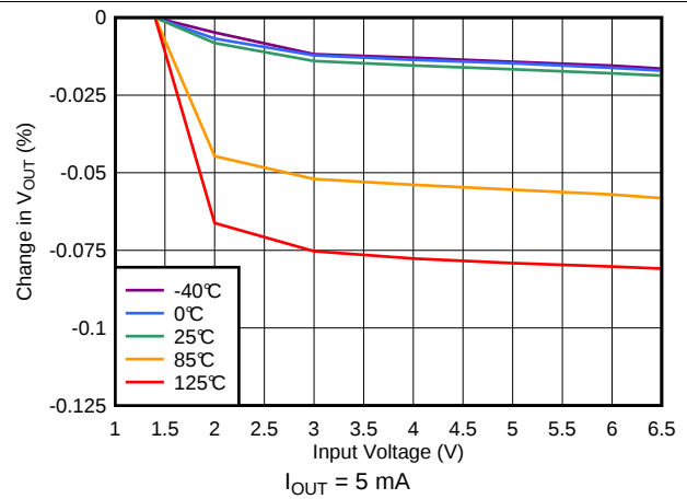
图 32. Line Regulation without Bias
