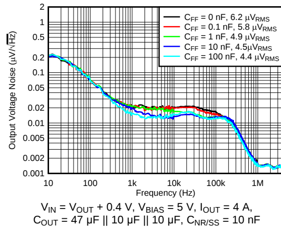
图 15. Output Noise vs Frequency and C_{FF}
