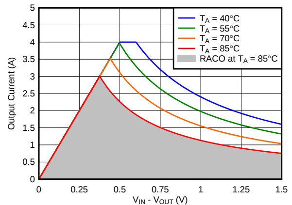
图 64. Recommended Area for Continuous Operation for V_{OUT} = 5.0\text{ V}
