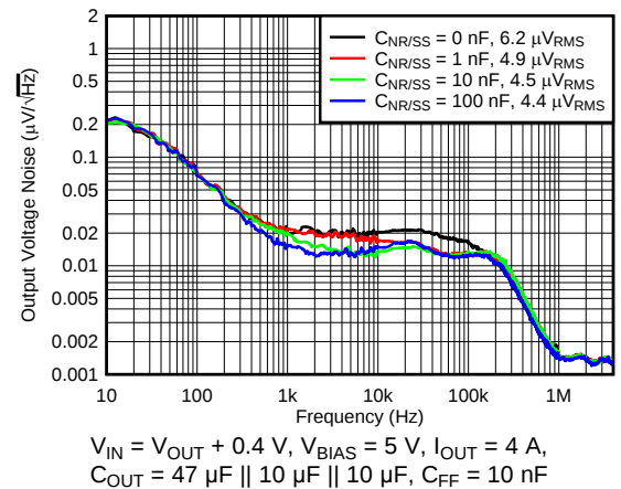
图 14. Output Noise vs Frequency and C_{NR/SS}
