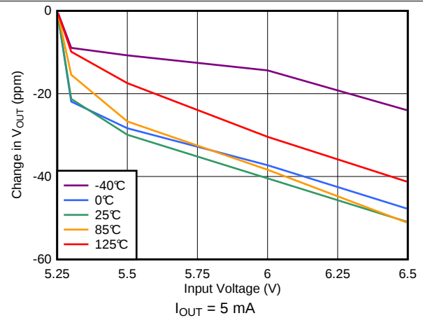
图 34. Line Regulation (5-V Output)
