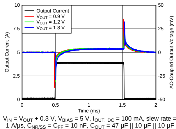
图 18. Load Transient Waveform vs Time and V_{OUT} with Bias
