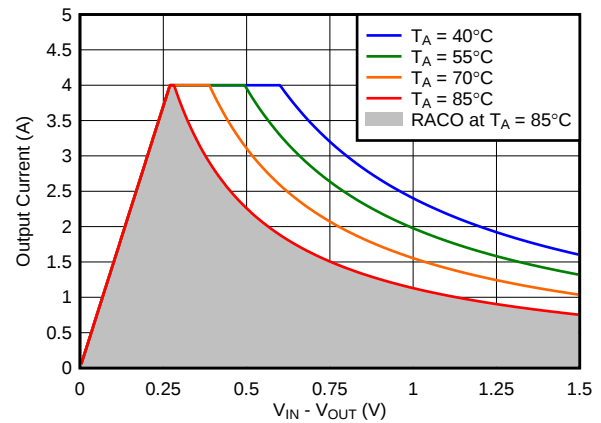
图 62. Recommended Area for Continuous Operation for V_{OUT} = 2.5\text{ V}
