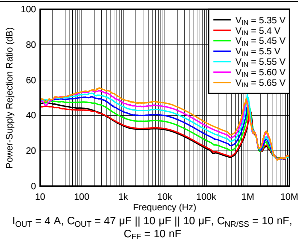
图 9. PSRR vs Frequency and V_{IN} for V_{OUT} = 5.0\text{ V}
