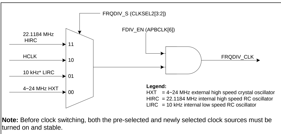
Figure 6-8 Clock Source of Frequency Divider
