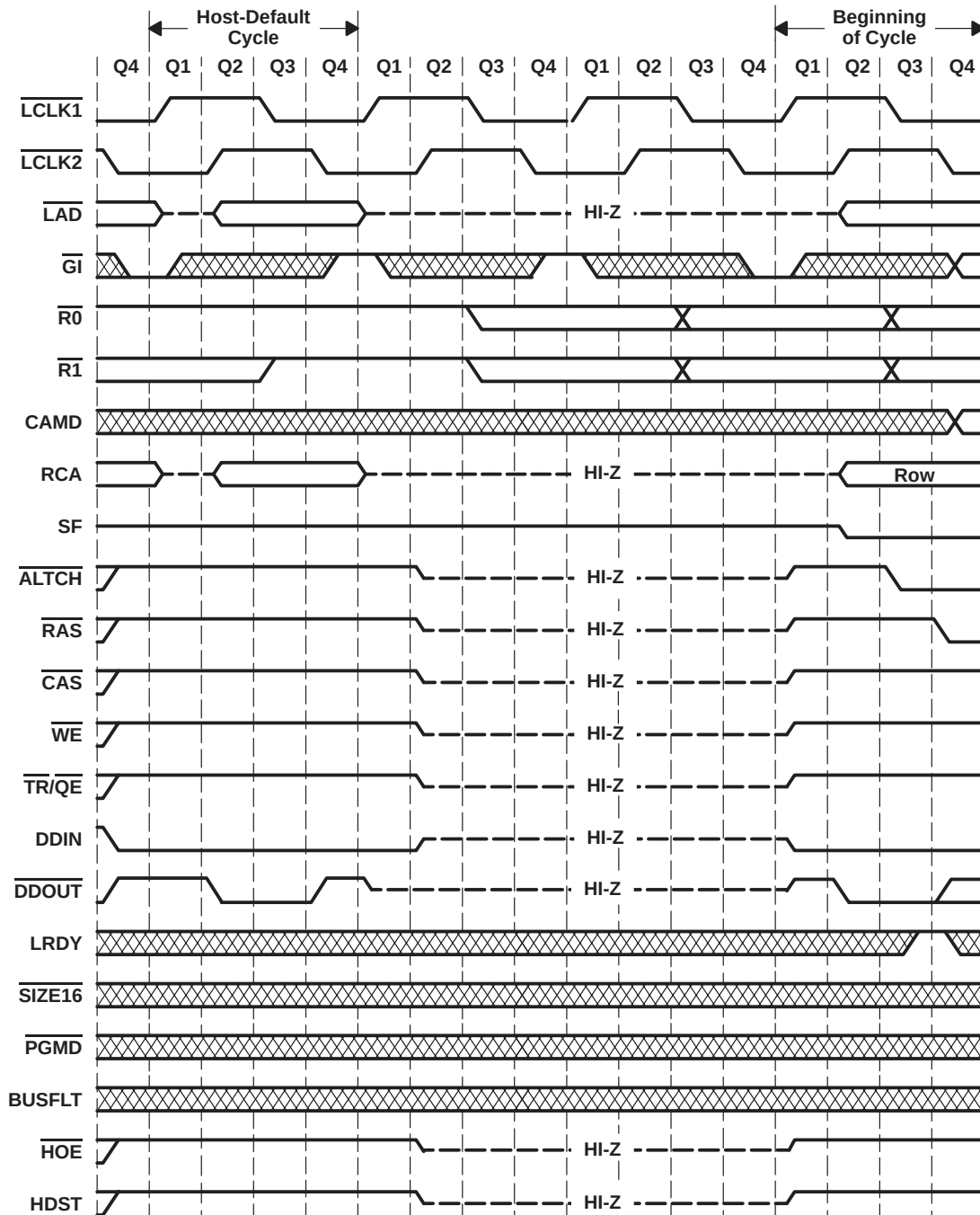
Figure 18. Multiprocessor Interface Timing (High-Impedance Signals)
