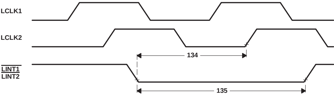
Figure 49. Interrupt Timing: \overline{\text{LINT1}} and \overline{\text{LINT2}}
