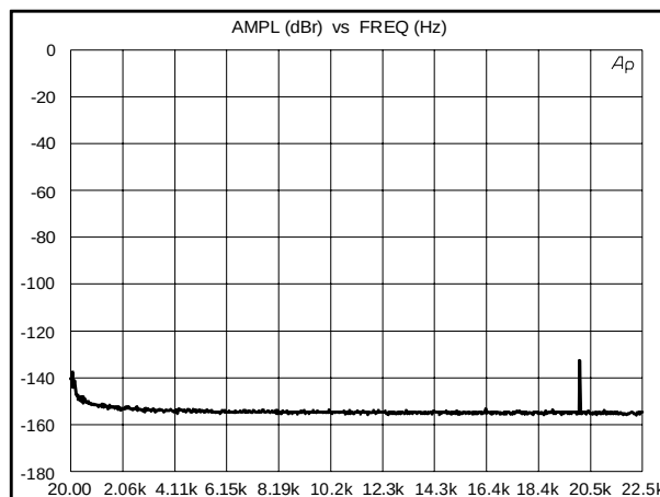
Figure 7. 20 kHz Crosstalk
