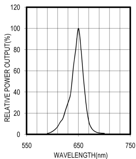
SPECTRAL OUTPUT
