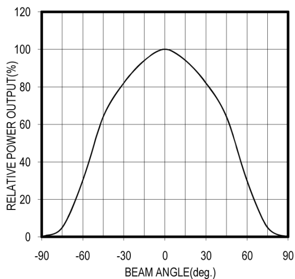
RADIATION PATTERN
