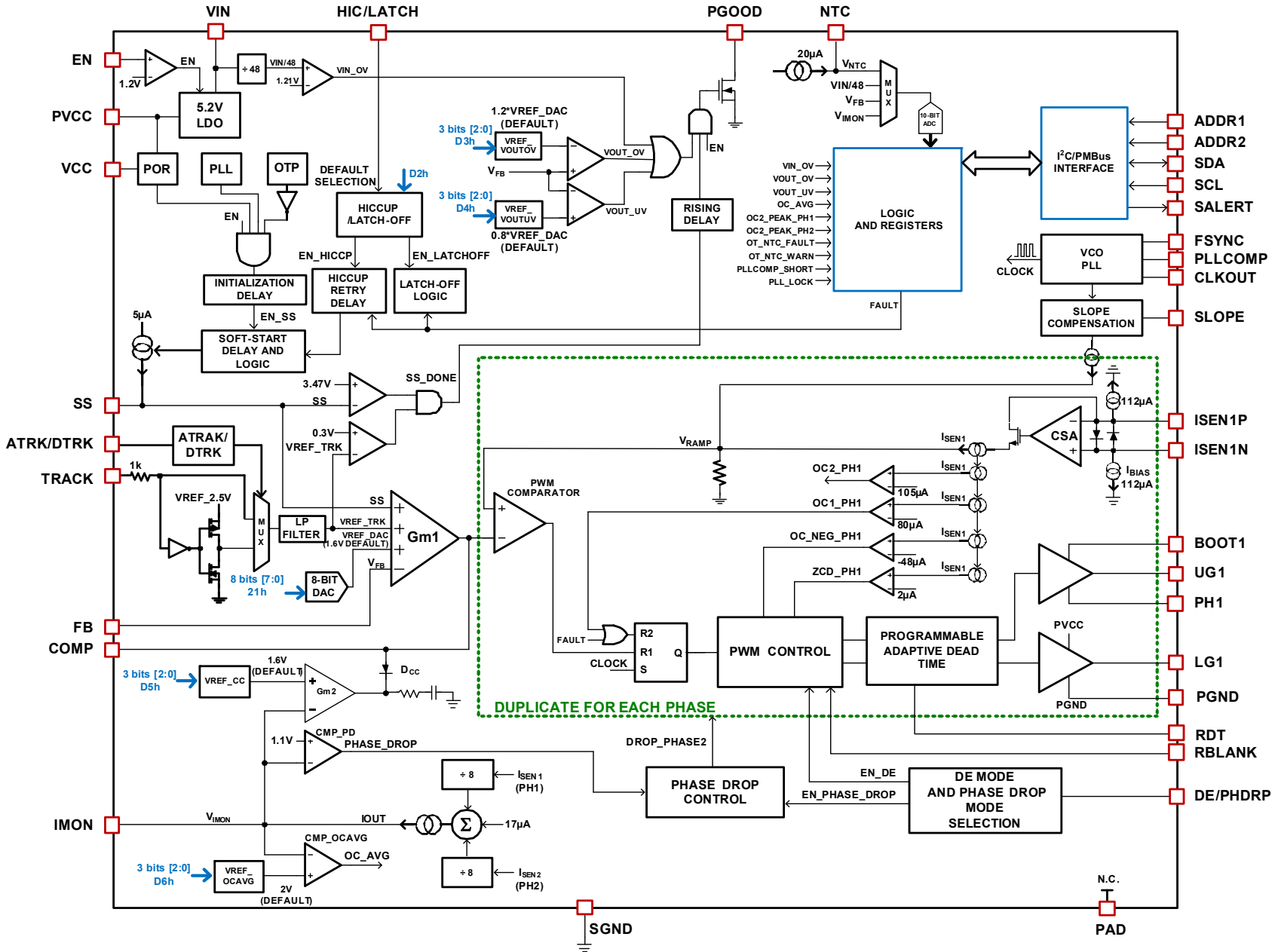
FIGURE 3. BLOCK DIAGRAM
