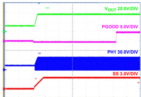
FIGURE 8. SOFT-START, CCM MODE (DE/PHDRP = GND), I_{OUT} = 8A
