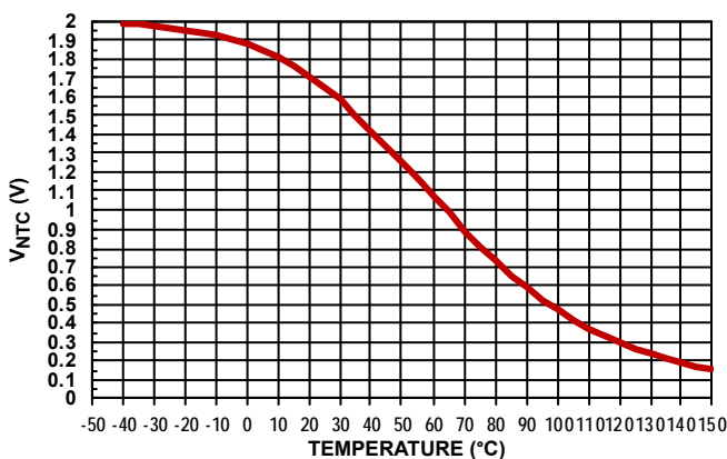
FIGURE 71. NTC VOLTAGE vs TEMPERATURE
