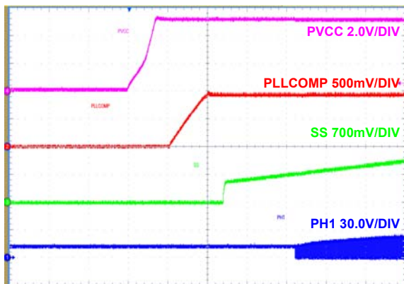
FIGURE 7. EN ON AND INITIALIZATION TO START-UP, I_{OUT} = 0A
