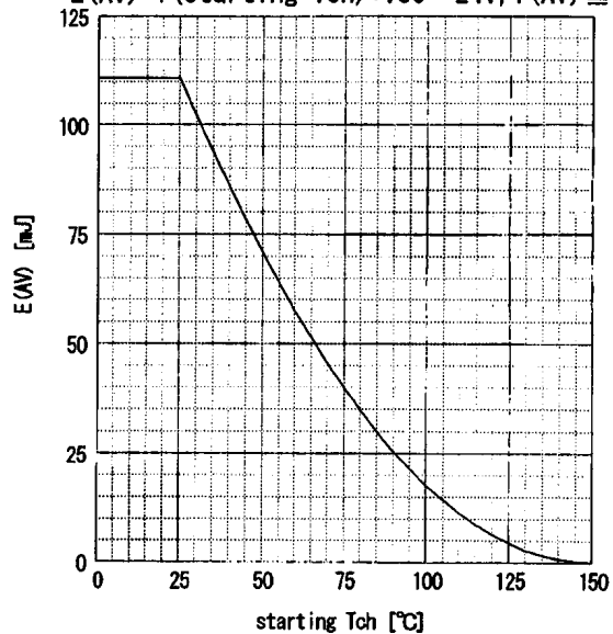
Maximum Avalanche Energy vs. starting T_{ch} E_{(AV)} = f(\text{starting } T_{ch}) : V_{GS} = -24V, I_{(AV)} \geq -7A
