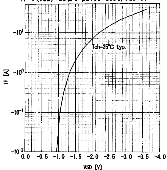
Forward characteristic of reverse of diode
