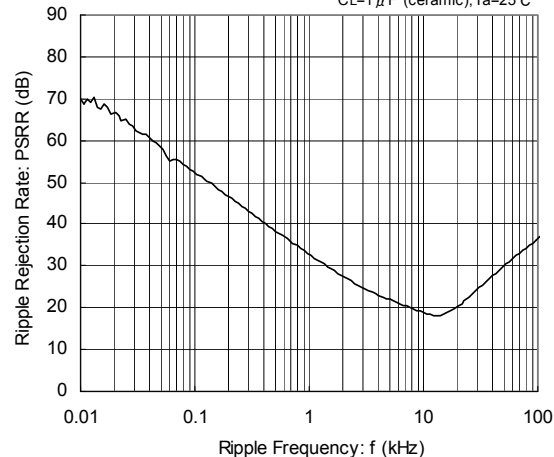
XC6216B/D 502
