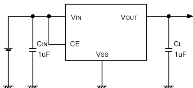
Fixed Output Voltage XC6216B/XE6216B Series
