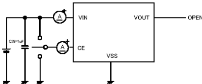
Circuit ②
