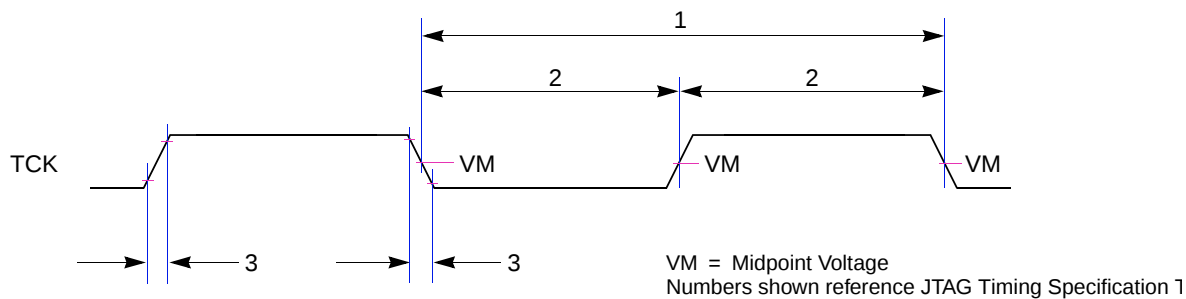
Figure 45. Timing Diagram — JTAG Clock Input
