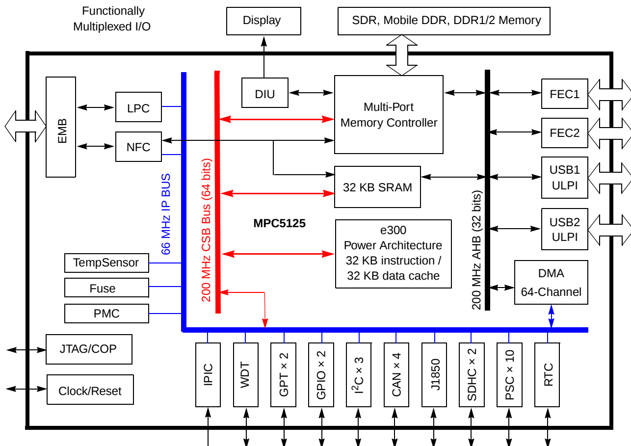
Figure 2. Simplified MPC5125 Block Diagram
