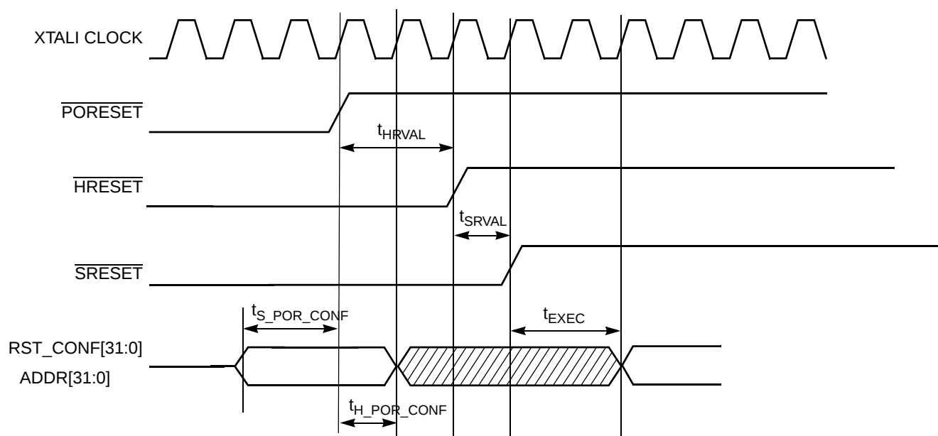
Figure 5. Power-Up Behavior
