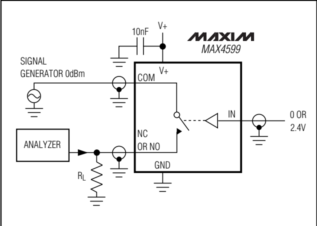
Figure 5. Off-Isolation/On-Channel Bandwidth
