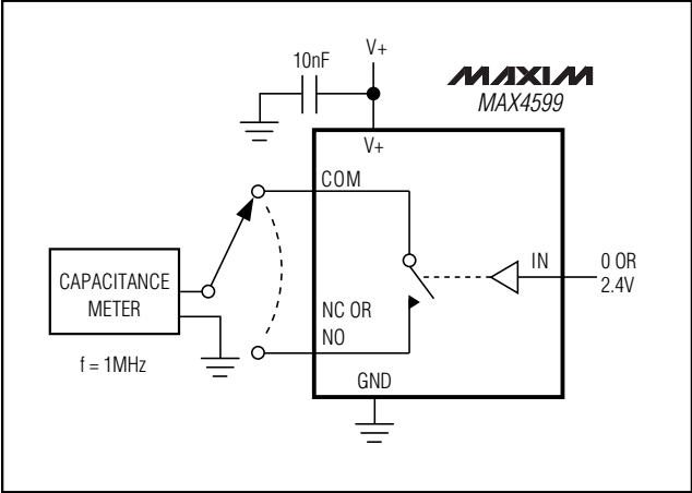
Figure 6. Channel On/Off-Capacitance
