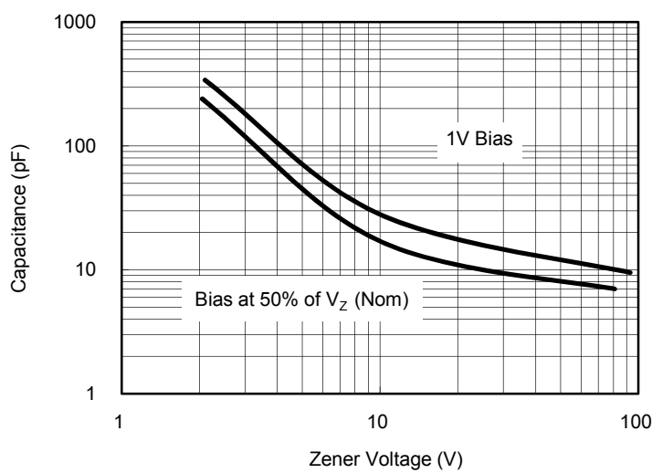
Fig. 5 Typical Capacitance
