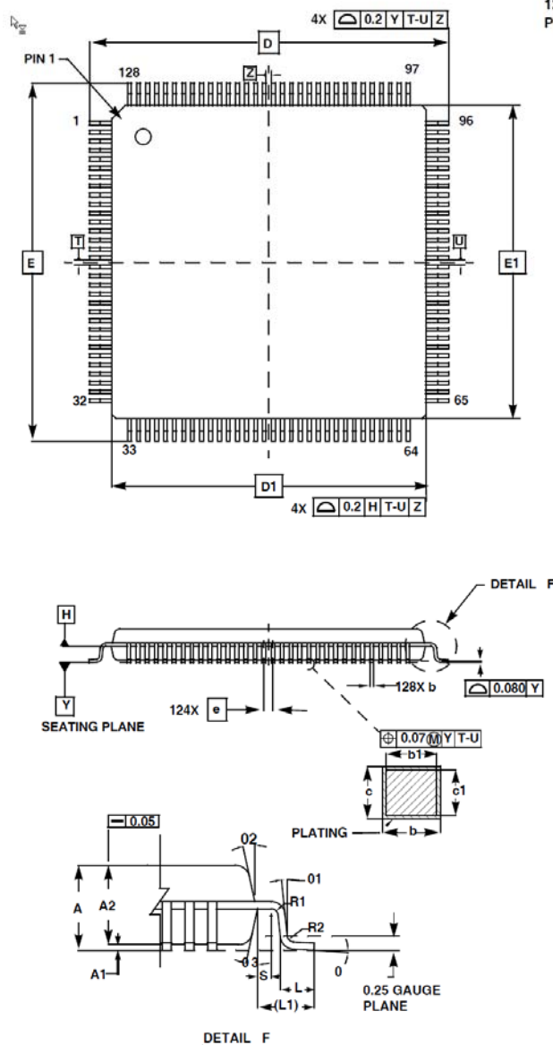
Figure 3-2 : RA8876 Package Outline Dimensions
