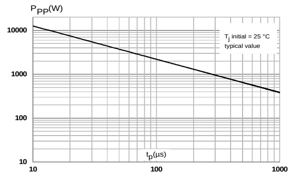
Figure 4: Peak pulse power versus exponential pulse duration ( T_J = 25^\circ\text{C} , typical value)
