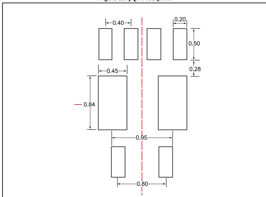
Figure 10: \mu QFN footprint
