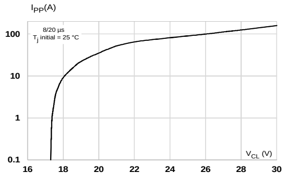
Figure 5: Peak pulse current versus clamping voltage (max. value)
