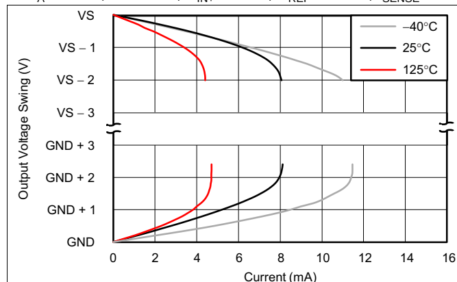
Figure 19. Output Voltage Swing vs Output Current
