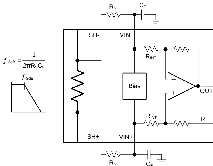
Figure 33. Input Filter
