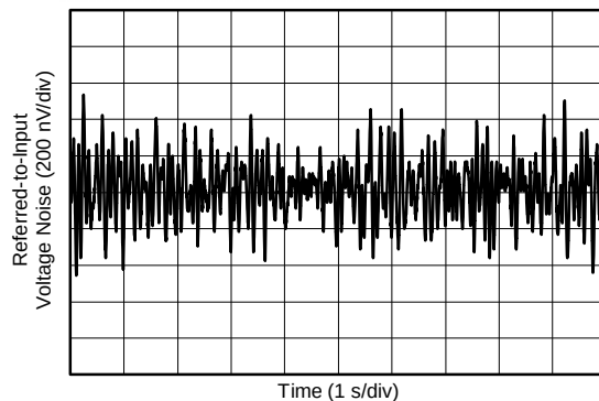
Figure 26. 0.1-Hz to 10-Hz Voltage Noise (Referred-to-Input)
