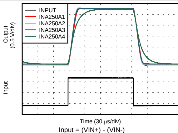
Figure 27. Step Response
