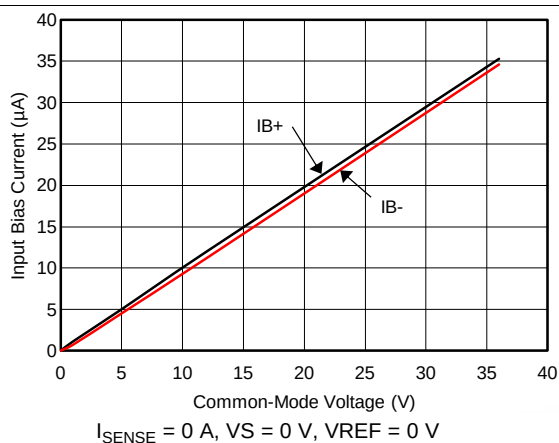
Figure 21. Input Bias Current vs Common-Mode Voltage (VS = 0 V)
