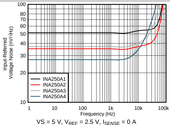
Figure 25. Input-Referred Voltage Noise vs Frequency
