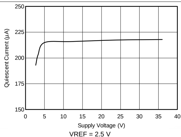
Figure 24. Quiescent Current vs Supply Voltage
