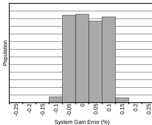
Figure 14. System Gain Error Distribution
