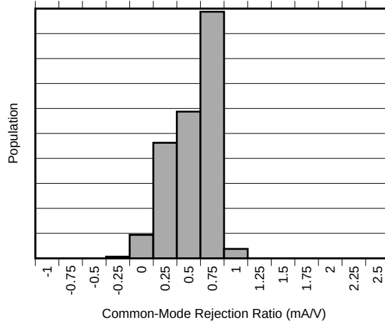
Figure 7. INA250A2 Common-Mode Rejection Ratio Distribution
