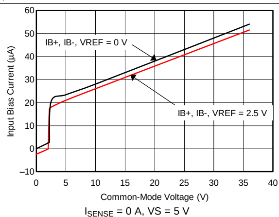
Figure 20. Input Bias Current vs Common-Mode Voltage (VS = 5 V)
